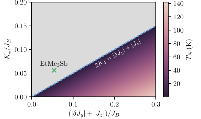
FIG. 4. Numerical calculation of the ordering temperature as a function of the interchain ring exchange, K_4 , and the unfrustrated interchain couplings, \delta J_y and J_z . Our calculated parameters for EtMe 3 Sb are marked by the green cross. We have used our calculated values for the other couplings in Eq. (2); \bar{J}_y = 135 K, K_3 = 18 K, K'_4 = 76 K, and K''_4 = 66 K. The gray area indicates where there is no real positive solution for T_N . This occurs when 2K_4 > |\delta J_y| + |J_z| (as shown with the blue dashed line). For all points on this graph, k_0 and k_y + \pi/2 are both less than 10^{-4} .
