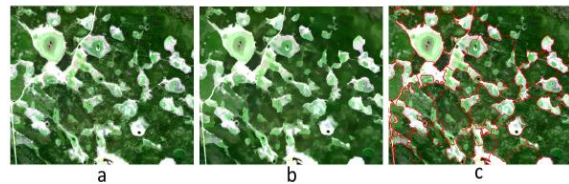
Figure 6. Object recognition from Sentinel 2A (a) RGB of PCA components; (b) MeanShiftSmoothing filtering; (3) Image segmentation of alas.
