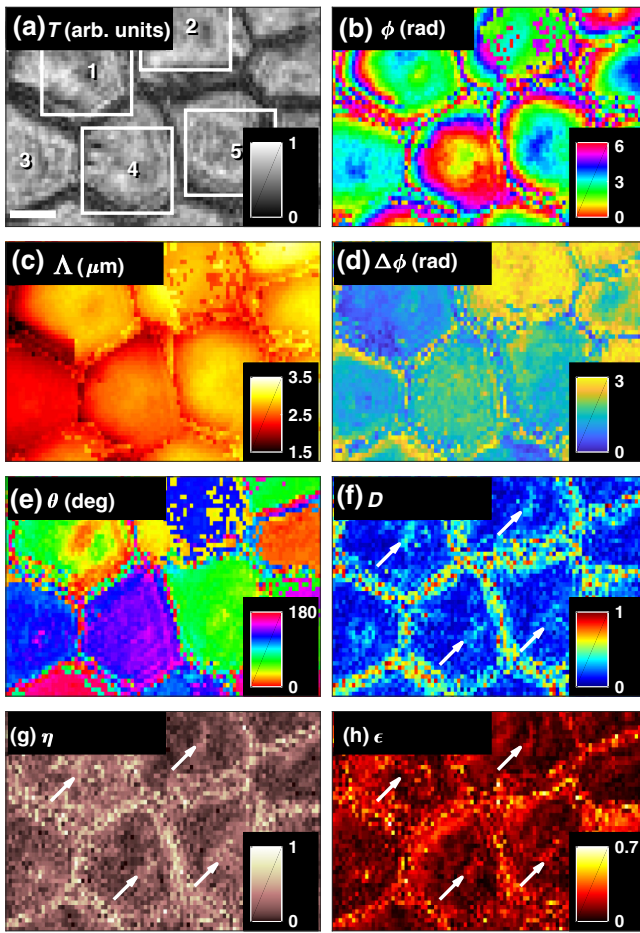
FIG. 3. Optical and structural properties retrieved from the framed area of the Jones maps in Fig. 2. The scale bar is 10 \mu\text{m} .
