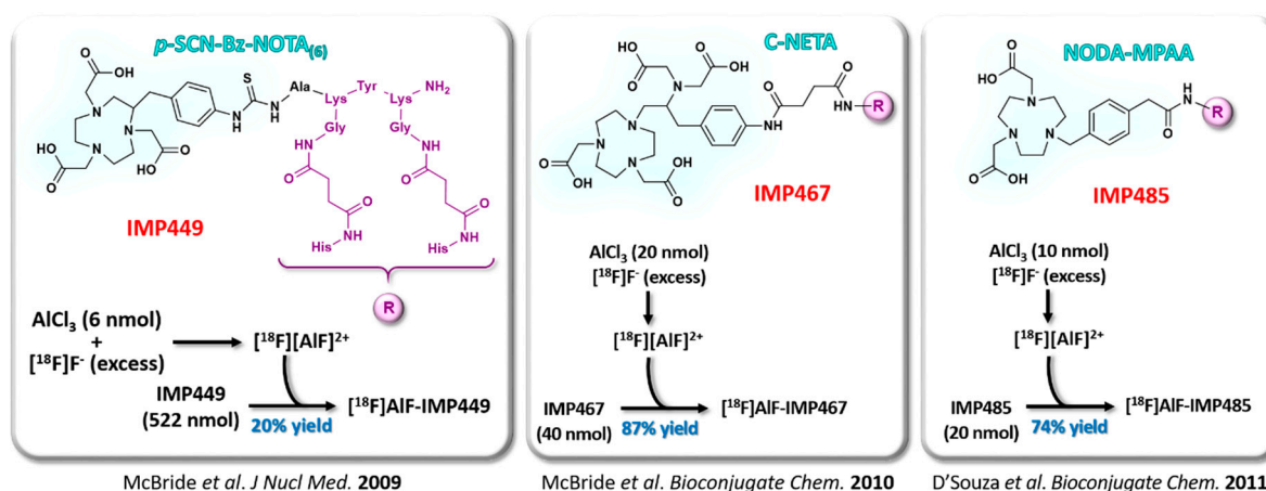
Figure 5. Structure and simplified radiofluorination protocols of the first [ ^{18}\text{F} ]AlF-labeled peptides.
