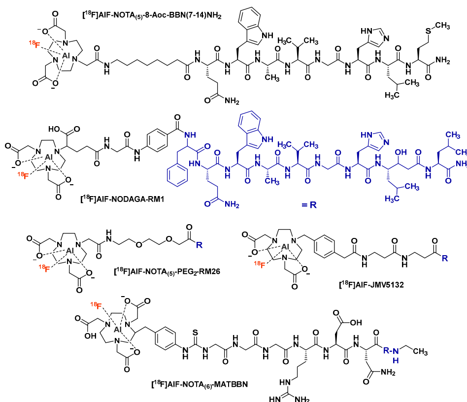
Figure 9. Chemical structures of several [^{18}\text{F}]\text{AlF} -labeled bombesin (BBN) analogs.
