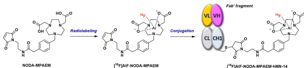
Figure 14. ^{18}\text{F} AIF radiolabeling and conjugation of NODA-MPAEM to a Fab' fragment.
