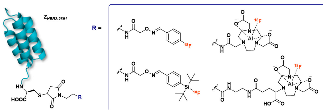
Figure 15. Schematic structures of ^{18}\text{F} -radiolabeled Z_{\text{HER2}:2891} affibodies studied by Glaser et al.
