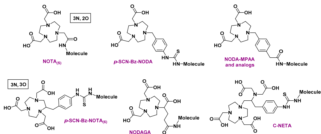
Figure 3. Examples of pentadentate or hexadentate bifunctional chelators used to radiolabel molecules with ^{18}\text{F}]\text{AlF} .
