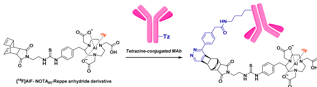
Figure 18. Pretargeting approach proposed by Shi et al. involving an [^{18}\text{F}]\text{AlF-NOTA}_{(6)} -Reppe anhydride derivative and Tz-conjugated MABs.
