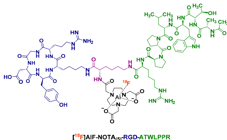
Figure 7. Chemical structure of ^{18}\text{F} -AIF- \text{NOTA}_{(5)} -RGD-ATWLPPR heterodimeric radioconjugate.
