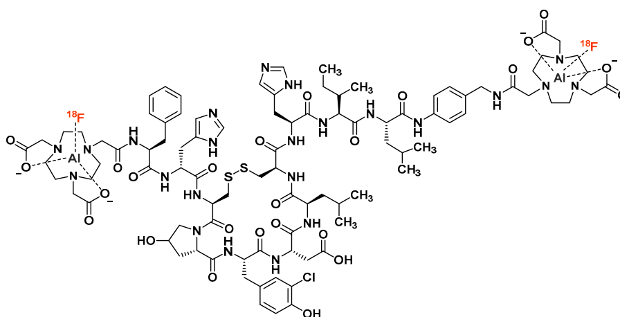
Figure 13. Chemical structure of bis- [^{18}\text{F}]\text{AlF-NOTA}_{(5)} fibrin-binding positron emission tomography (PET) probe.
