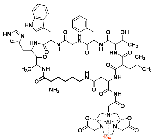
Figure 11. Chemical structure of [ ^{18}\text{F} ]AlF-NOTA (5) -C6.
