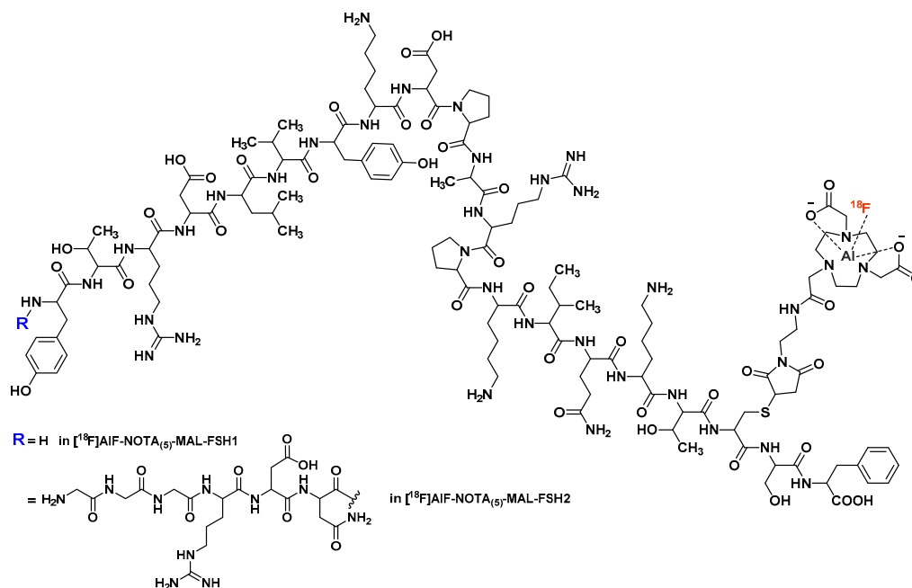
Figure 10. Chemical structures of [^{18}\text{F}]\text{AlF-NOTA}_{(5)}\text{-MAL-FSH1} and [^{18}\text{F}]\text{AlF-NOTA}_{(5)}\text{-MAL-FSH2} .
