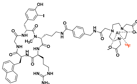
Figure 12. Chemical structure of [^{18}\text{F}]\text{AlF-NOTA}_{(5)} -Pentixather.
