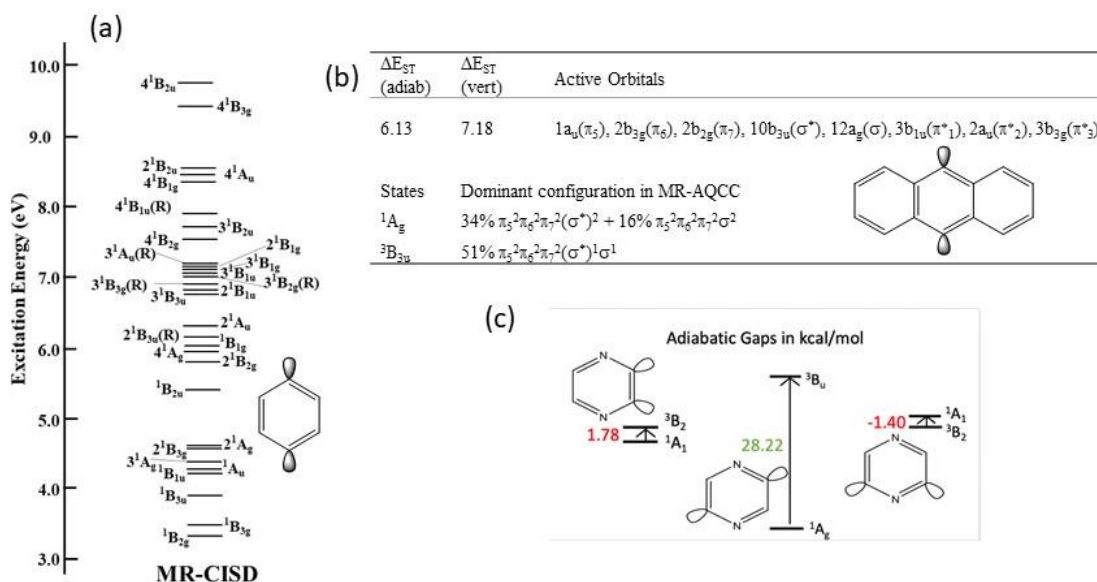
Fig. 2 (a) 32-state averaged CAS(8,8) MRCI/TZ energy diagram for para -benzyne showing densely packed manifold of singlet excited valence and Rydberg states within a 10 eV window of the singlet 1A_g ground state. (b) MR-AQCC/DZ adiabatic and vertical excitation energies (kcal/mol) for the anthracene diradical using the CAS (8,8) active space. Electron configurations
