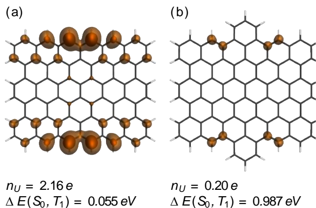
Fig. 4 MRCI computations on two different graphene nanoflakes: (a) a periacene with an unperturbed zig-zag edge and (b) the same system with two additional phenyl rings. The contour plots represent the distribution of unpaired electrons (isovalues 0.005/0.0005 a.u.).
