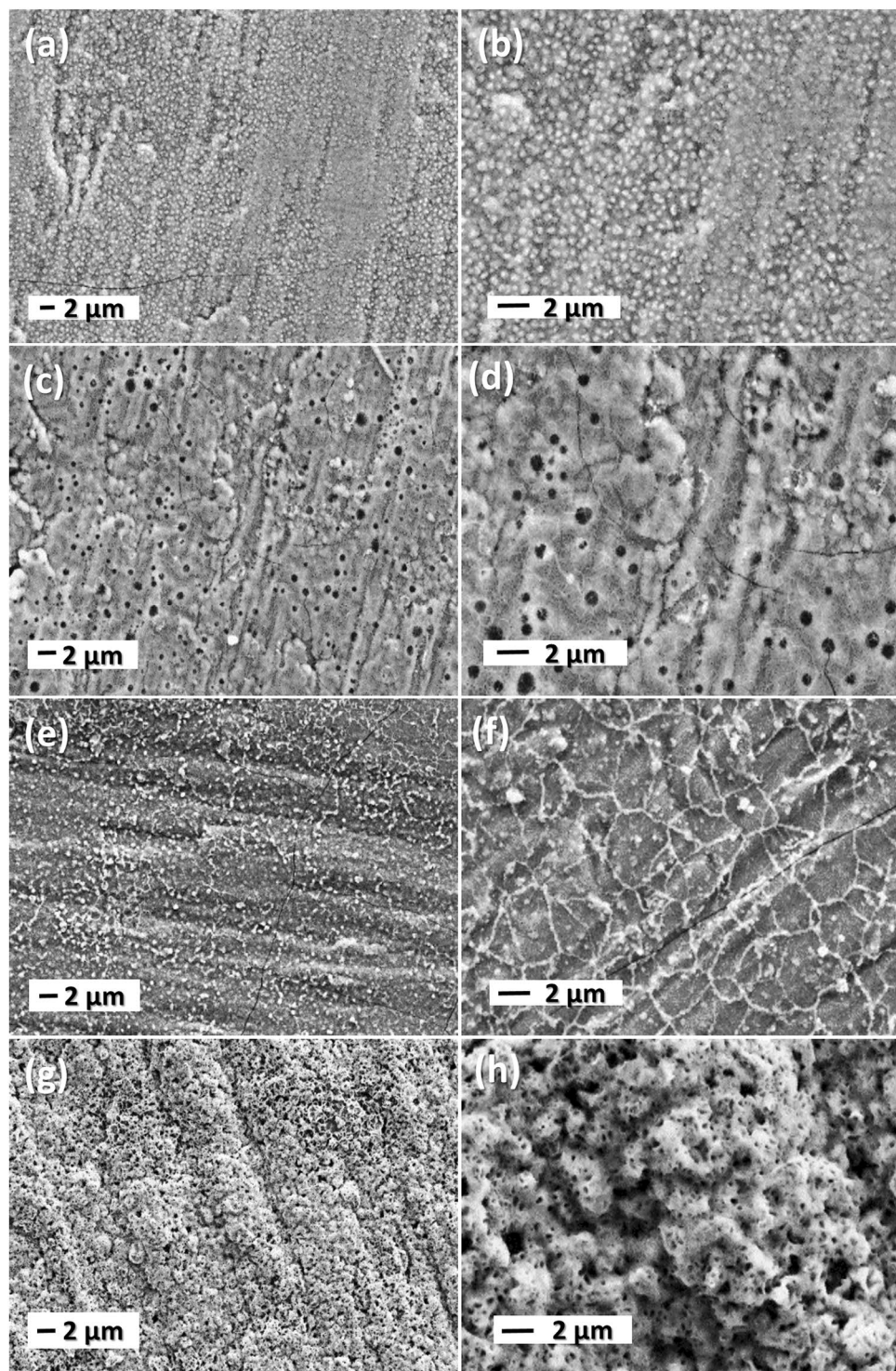
Figure 5. SEM images the annealed films at different temperatures LFP-400 (a,b), LFP-500 (c,d), LFP-600 (e,f) and LFP-700 (g,h).
