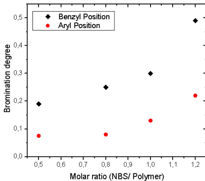
Fig. 3. Bromination degree of PPO in the different positions as function of molar ratio NBS/Polymer.
