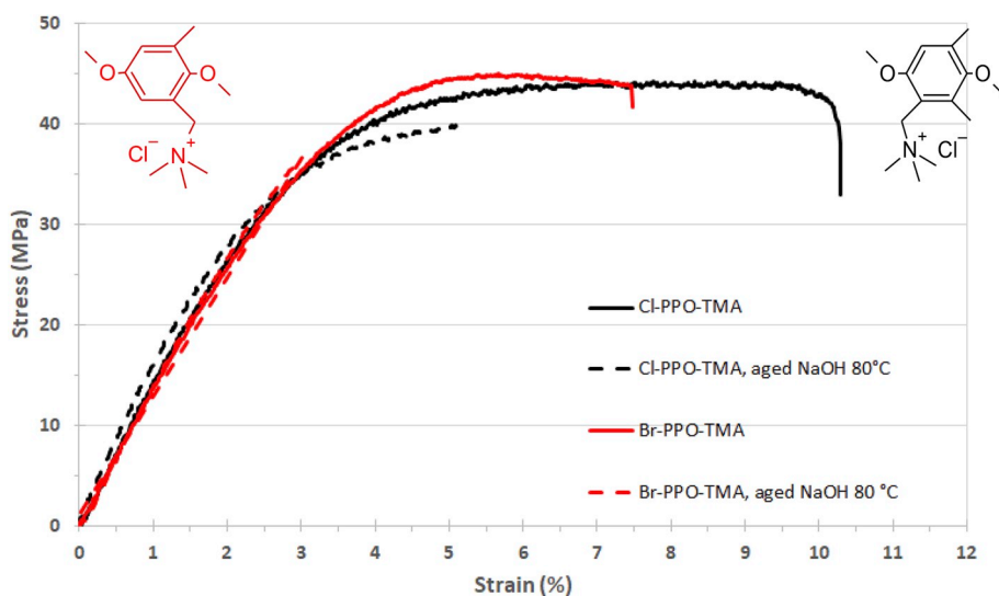
Fig. 10. Stress-strain tests at room temperature and ambient humidity (50 ± 10% RH) of AEM (chloride form, initial IEC = 1.6 meq/g) before and after aging in NaOH at 80 °C (72 h).
