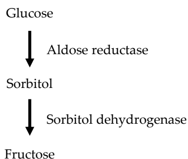
Figure 2. The polyol pathway. The polyol pathway is a two-step enzymatic pathway. In the first step, glucose is reduced to sorbitol by aldose reductase. In the second step, sorbitol is converted to fructose by sorbitol dehydrogenase. Endothelial toxicity arises from sorbitol/fructose accumulation within endothelial cells.
