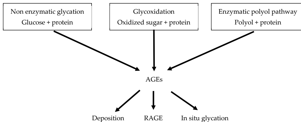
Figure 3. The major biomechanisms leading to the formation of advanced glycation end products (AGEs).
