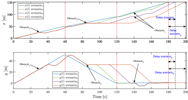
Fig. 6. x(t) and y(t) trajectories of all the studied scenarios.
