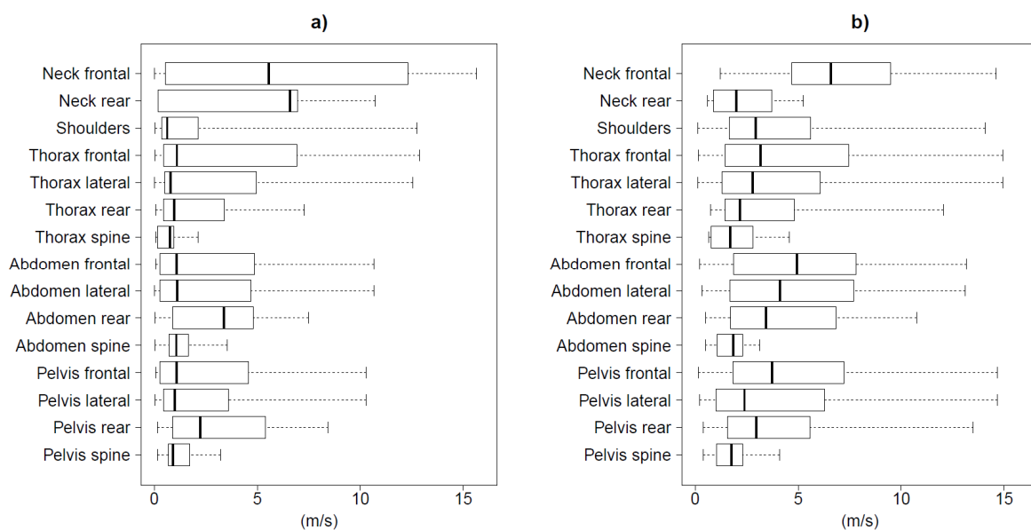
Figure 6. Impact velocity distribution for each trunk region with the car. a) Normal component. b) Tangential component.
