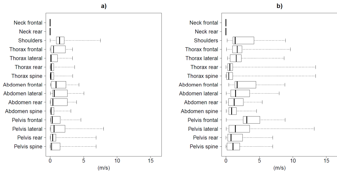
Figure 7. Impact velocity distribution for each trunk region with the ground. a) Normal component. b) Tangential component.
