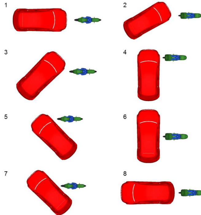
Figure 3. PTW-car collision points representing the simulated scenarios: Head-on (1), head-on 150° (2), oblique-on-side 135° at front wheel level (3), head-on-side at front wheel level (4), oblique-on-side 45° at front wheel level (5), head-on-side at B-pillar level (6), oblique-on-side 45° at B-pillar level (7) and head-on-rear (8).
