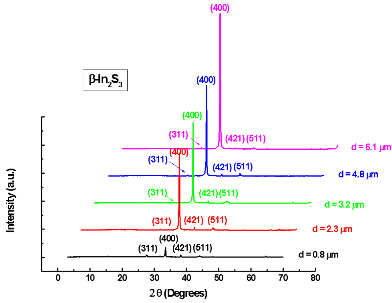
Fig. 2: XRD patterns of sprayed \text{In}_2\text{S}_3 films.
