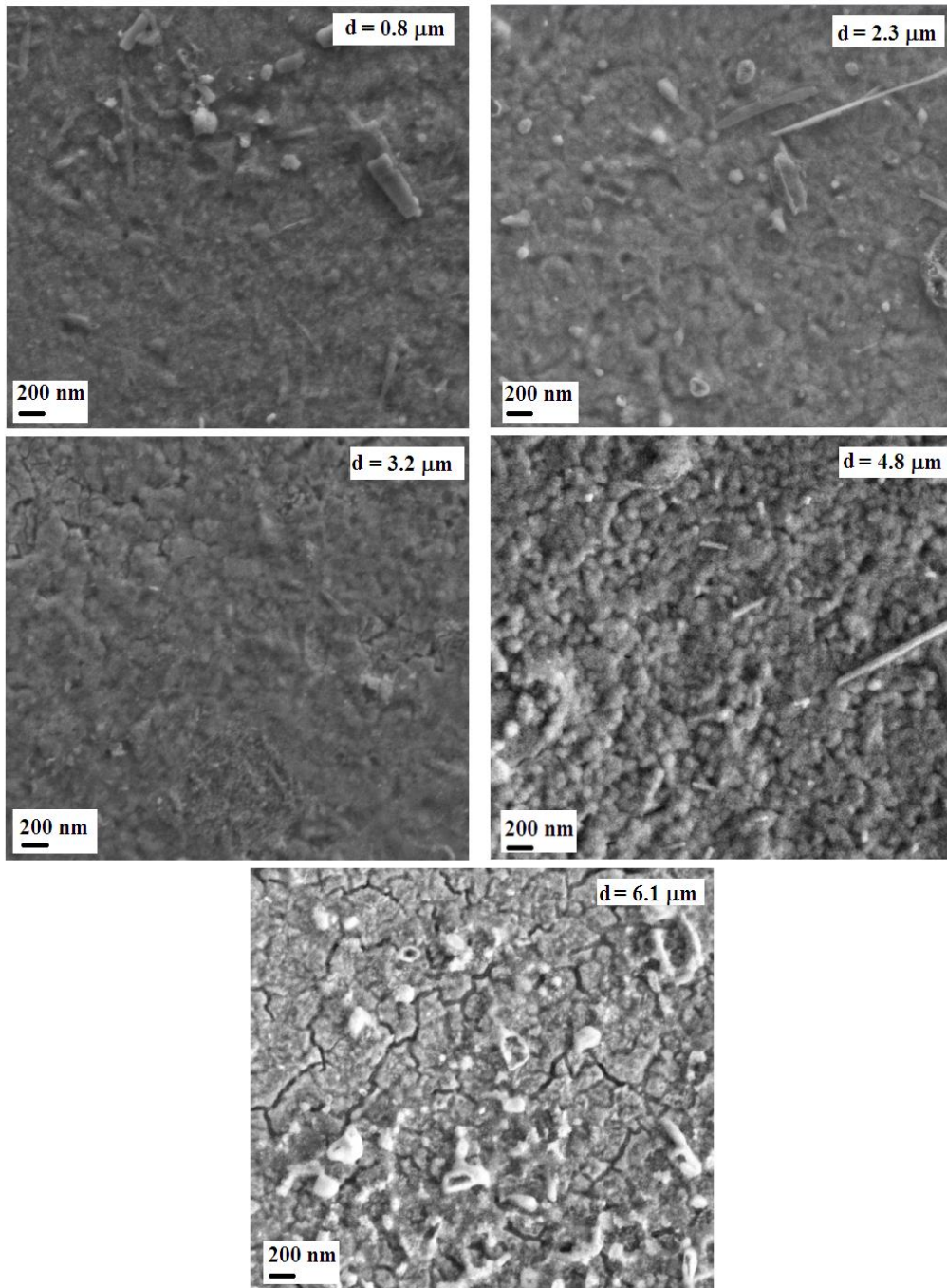
Fig. 4: SEM images of sprayed \text{In}_2\text{S}_3 films.
