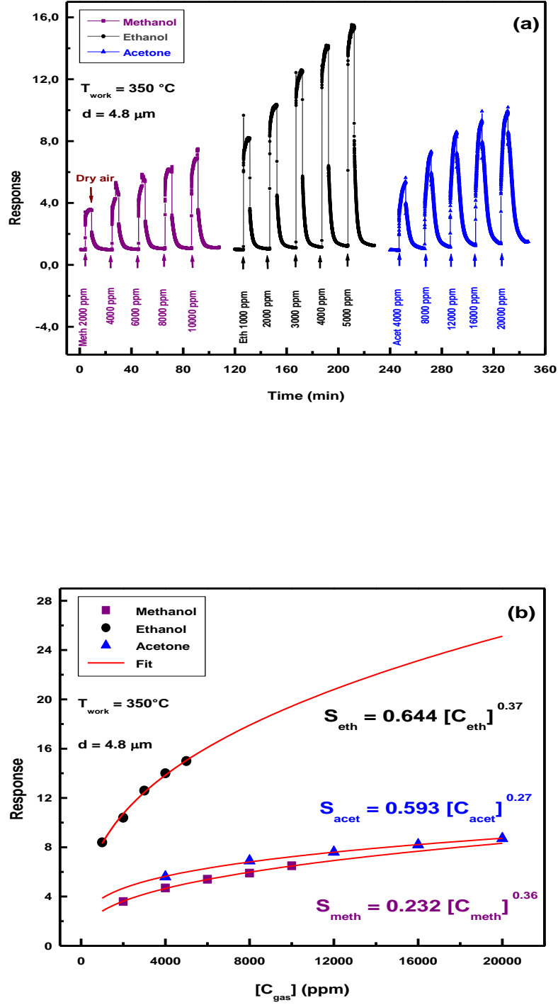
Fig. 10: (a) Dynamic response of \text{In}_2\text{S}_3 sensor to various organics vapors concentrations at 350^\circ\text{C} , (b) experimental and power fit of sensing response of \text{In}_2\text{S}_3 sensor as a function of organic vapor concentration at 350^\circ\text{C} .
