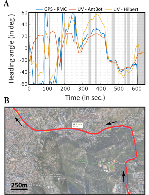
Fig. 5. A Heading angle (in degrees) estimated over the Luminy road, according to the first dataset (06-2018; f_{COMP} = 0.077\text{Hz} ). Gray areas depict the moments when the GPS was unavailable. B Sky view of the trajectory.
