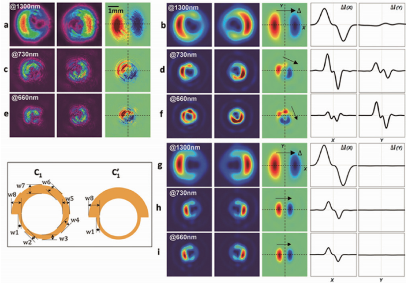
Figure 6: Wavelength-dependence of a spin-dependent beam separation. Wavelength-dependence of a spin-dependent beam separation in C_{1h} TA-CGSM metasurface is shown at 1300 nm, 730 nm, and 660 nm. (a), (c), (e), Experimental measurements and (b), (d), (f), FDTD calculations for C_{1h} TA-CGSM. g, h, i, FDTD calculations for C'_{1h} metasurface with incident Gaussian beam propagation along +z .
