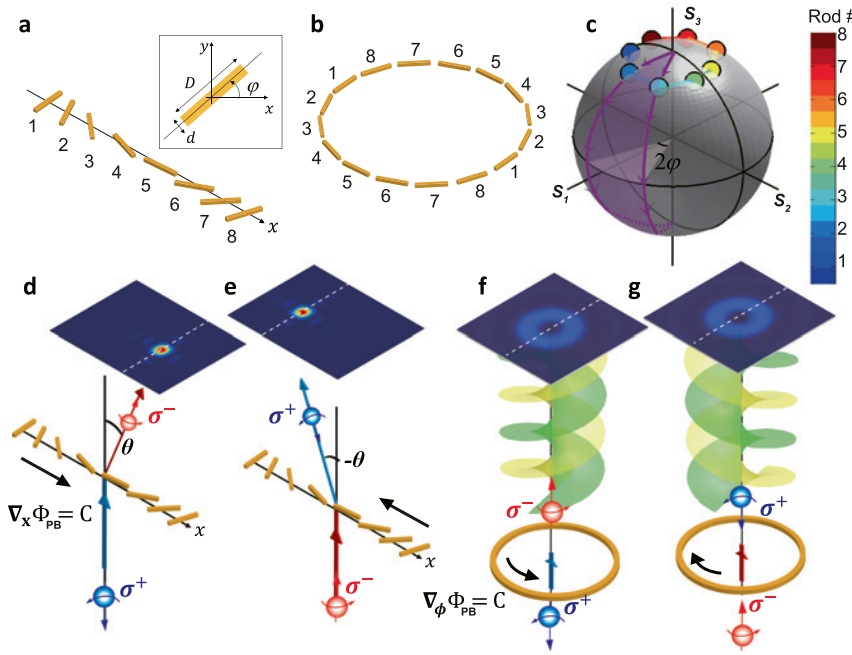
Figure 1: Array of nano-rods with a constant gradient PB phase and Poincaré sphere plot of Stokes parameters. Inset figure shows a schematic of nano-rod with length D and width d making an angle \phi with x -axis. (a) Linear array of rotating nano-rods from one to eight. (b) Circular array of nano-rods from one to eight in the range of 0 \leq \phi \leq \pi and repeated in the range of \pi \leq \phi \leq 2\pi . (c) Poincaré sphere plot of Stokes parameters of optical beams scattered from nano-rods of (a) and (b) for LCP incident beam. Color code corresponds to the nano-rod number. (d, e) Spin-dependent beam deflection of cross-polarization scattered optical beam shown up as a spin-dependent beam separation. +x -direction deflection of RCP \sigma^- beam for LCP \sigma^+ incidence beam in (d) and whereas the opposite in (e). (f, g) Generation of vortex beam of topological charge l = \pm 2 . Topological charge l = +2 with polarization state of RCP \sigma^- for LCP \sigma^+ Gaussian incidence beam in (f), and topological charge l = -2 with polarization state of LCP \sigma^+ for RCP \sigma^- Gaussian incidence beam in (g).
