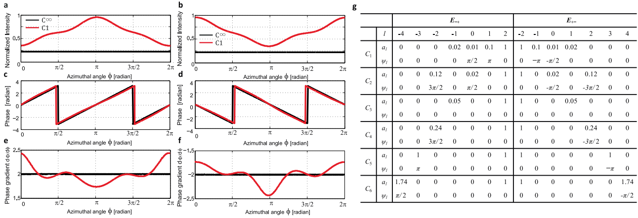
Figure 5: Analytically calculated intensity, phase, and phase gradient as a function of the azimuthal angle \phi . (a, b) Calculated far-field intensity I_{ij} . (c, d) Calculated phase \Phi_{ij} . (e, f) constant phase gradient d\Phi_{ij}/d\phi of C_{coh} (black) and nonuniform phase gradient of C_{1h} (red). The plots are for \{ij\} configuration, where \{ij\} are detection and incidence circular polarization helicity, \{-+\} for (a, c, e) and \{+-\} for (b, d, f). Non-constant phase gradient takes place owing to \phi -dependent \nabla_{\phi}\Phi_D(\phi) . (g) Fit values of partial-wave expansion coefficient \hat{a}_l , the l th order expansion coefficient.
