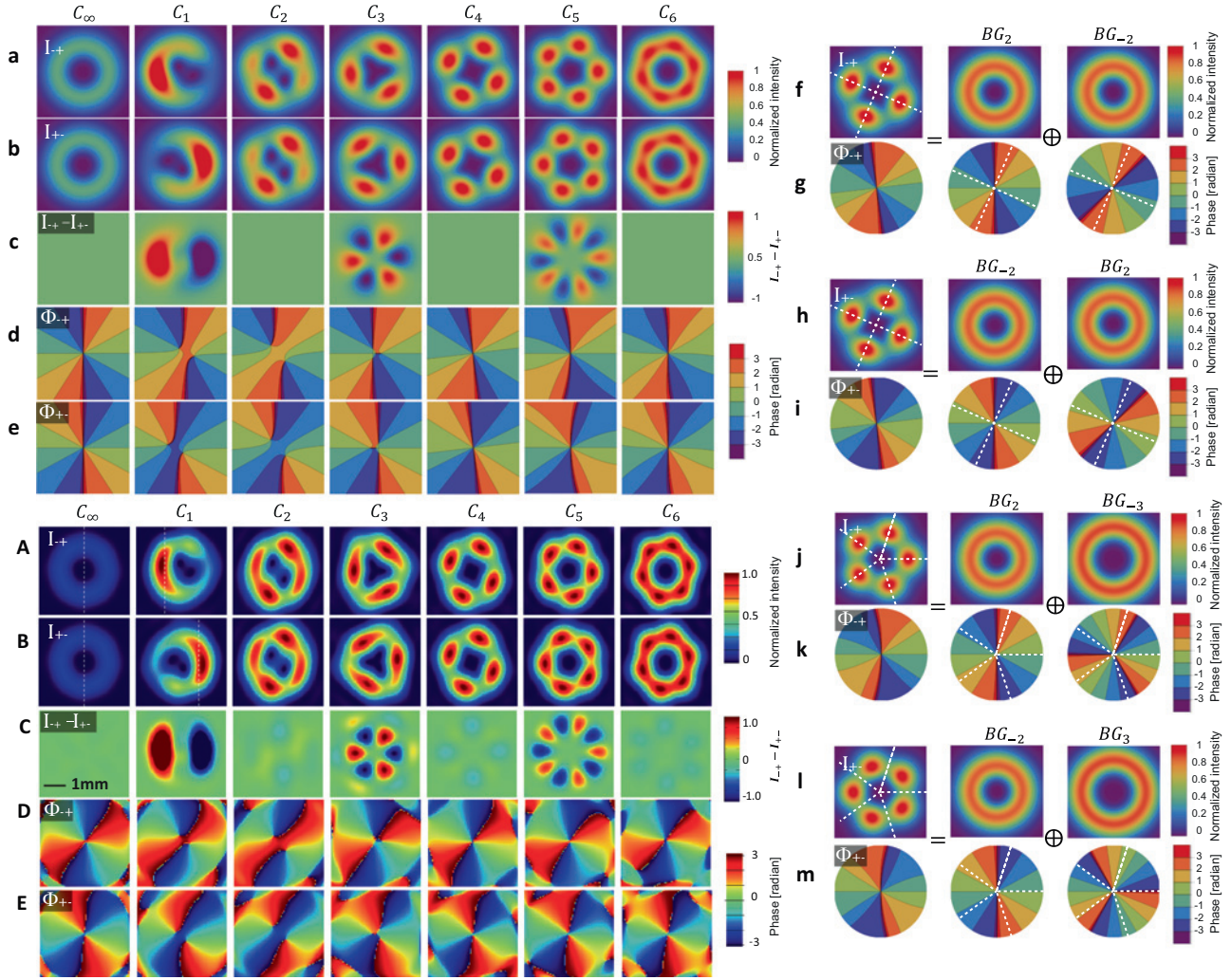
Figure 4: Analytical calculation and FDTD calculation of a spin-dependent beam separation for TA-CGSM. (a, b) Analytically calculated far-field intensity of I_{-+} and I_{+-} , respectively. (c) Calculated \Delta I = I_{-+} - I_{+-} . (d, e) Azimuthal distribution of phase for C_{coh} , C_1 , C_2 , C_3 , C_4 , C_5 , and C_6 TA-CGSM. (f-i) Partial-wave expansion of E_{-+} and E_{+-} of C_{4h} CGSM. (A, B) FDTD calculated far-field intensity of I_{-+} and I_{+-} , respectively. (C) Calculated \Delta I = I_{-+} - I_{+-} . (D, E) Azimuthal distribution of phase for C_{coh} , C_1 , C_2 , C_3 , C_4 , C_5 , and C_6 TA-CGSM. (j-m) Partial-wave expansion of E_{-+} and E_{+-} of C_{5h} CGSM.
