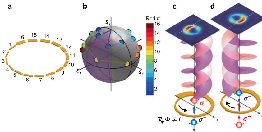
Figure 2: Circular array of nano-rods with a non-constant azimuthal gradient total phase and Poincaré sphere plot of Stokes parameters. (a) Circular array of nano-rods with varying width d from # 1 to # 16 in the range of 0 \leq \phi \leq 2\pi (b) Poincaré sphere plot of Stokes parameters of optical beams cross-polarization scattered from nano-rods of (a) for LCP \sigma+ incidence beam. Color code corresponds to the nano-rod number. (c, d) Generation of asymmetric vortex beam and spin-dependent beam separation. Bright and dark spots are separated along x -direction for both LCP \sigma+ in (c) and RCP ( \sigma- ) in (d) Gaussian incidence beams.
