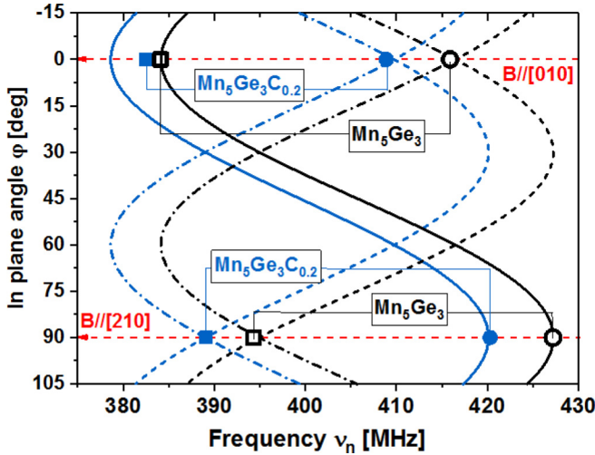
FIG. 8. Frequency branches of the NMR spectrum computed for three nonequivalent \text{Mn}_{II} positions (solid line denotes n = 1 , dashed line denotes n = 2 , dashed dot line denotes n = 3 ) as a function of orientation of the in-plane field in \text{Mn}_5\text{Ge}_3\text{C}_{0.2} (blue lines) and in the reference pristine \text{Mn}_5\text{Ge}_3 film (black lines): \nu_n(\phi) = \nu_{||} + \Delta\nu \sin^2[\phi + (n-1)60] - \gamma B_{\text{ext}} .
