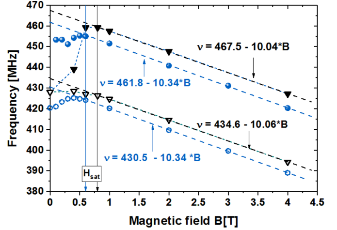
FIG. 9. NMR frequency of the two components of the ^{55}\text{Mn} NMR line from the \text{Mn}_{II} sites not having carbon nearest neighbors, observed at \phi = 90^\circ in \text{Mn}_5\text{Ge}_3\text{C}_{0.2} (blue spheres) and in the reference pristine \text{Mn}_5\text{Ge}_3 film (black triangles), plotted as a function of the in-plane field strength.
