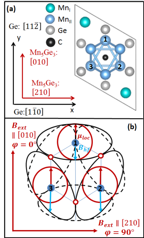
FIG. 5. (a) Projection of the atomic arrangement in the \text{Mn}_5\text{Ge}_3 unit cell on the (001) plane and the definition of the local coordinate system: The “x” axis ( \phi = 90^\circ ) is along the [210] direction of \text{Mn}_5\text{Ge}_3 parallel to the [1\bar{1}0] direction of the Ge substrate, the “y” axis ( \phi = 0^\circ ) is along [010] in \text{Mn}_5\text{Ge}_3 and [11\bar{2}] in Ge. Numbers 1, 2 and 3 denote the \text{Mn}_{II} atoms located on the same atomic plane ( z = 1/4 ); (b) schematic presentation of the amplitude of in-plane hyperfine fields on the planes z = 1/4 (solid black lines) and z = 3/4 (dashed black lines).
