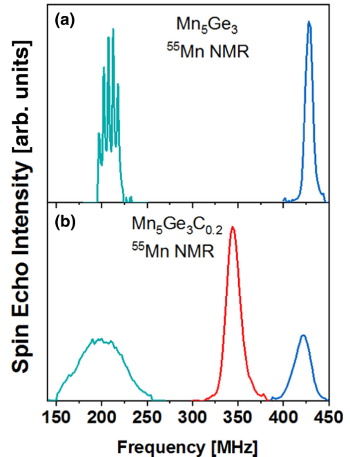
FIG. 2. Zero-field ^{55}Mn NMR spectra recorded at 4.2 K from the 300-nm films of Mn_5Ge_3 and Mn_5Ge_3C_{0.2} epitaxially grown on the Ge(111) substrate. Green: The NMR line from the Mn_I sites; blue: Mn_{II} sites with no carbon nearest neighbors; and red: Mn_{II} sites having carbon nearest neighbors.
