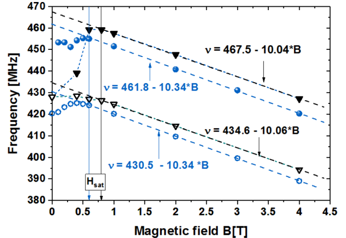
FIG. 9. NMR frequency of the two components of the ^{55}Mn NMR line from the Mn_{II} sites not having carbon nearest neighbors, observed at \phi = 90^\circ in Mn_5Ge_3C_{0.2} (blue spheres) and in the reference pristine Mn_5Ge_3 film (black triangles), plotted as a function of the in-plane field strength.
