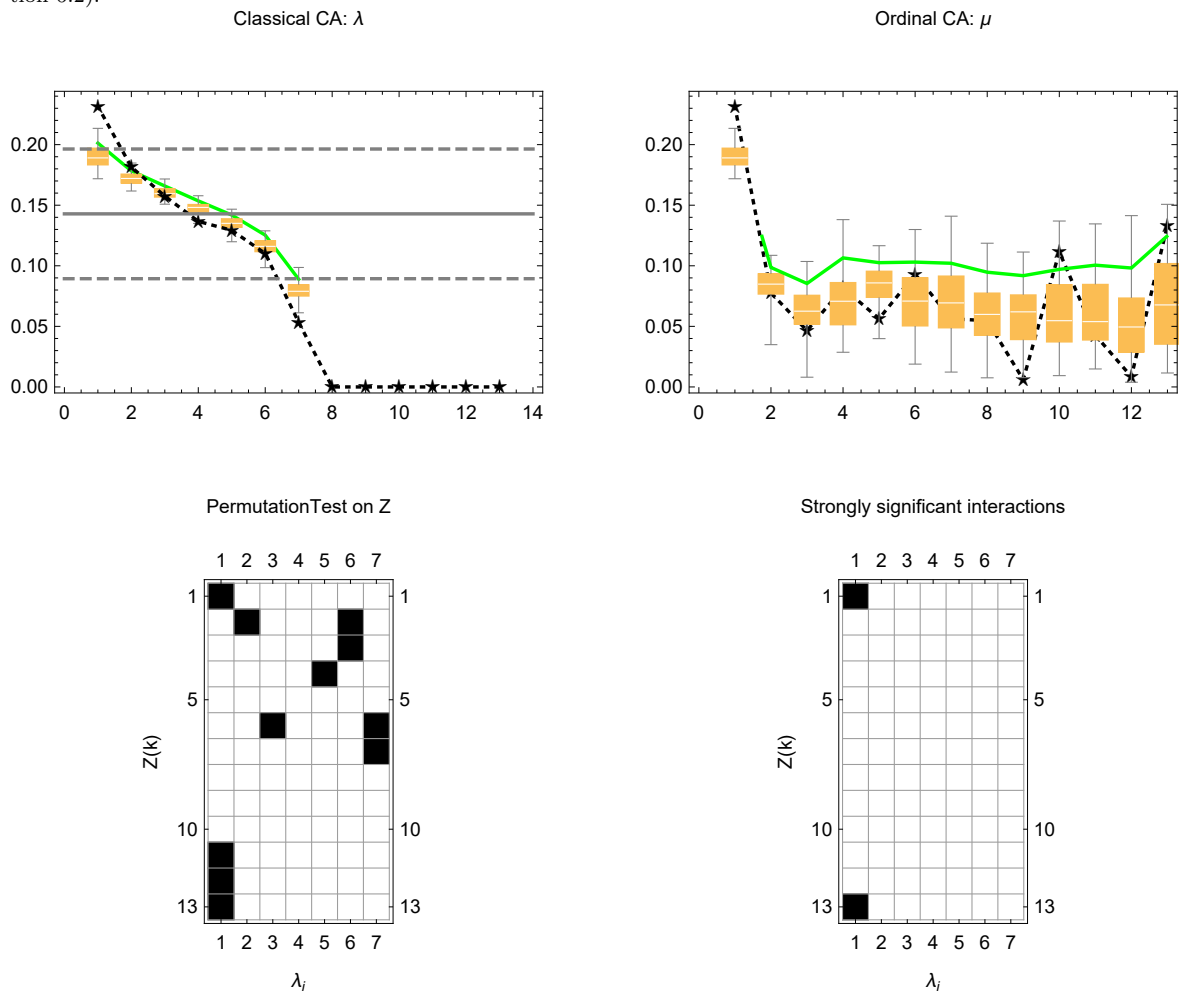
Figure 10. The X-rays diffraction data. Same structure as Figure 2. Upper plots: statistical significance of eigenvalues and polynomials coordinates. Lower plots, left panel: complete table of significant interactions (in black) issued from the permutation test; right panel (in black): strongly significant interactions (see Definition 6.2).
