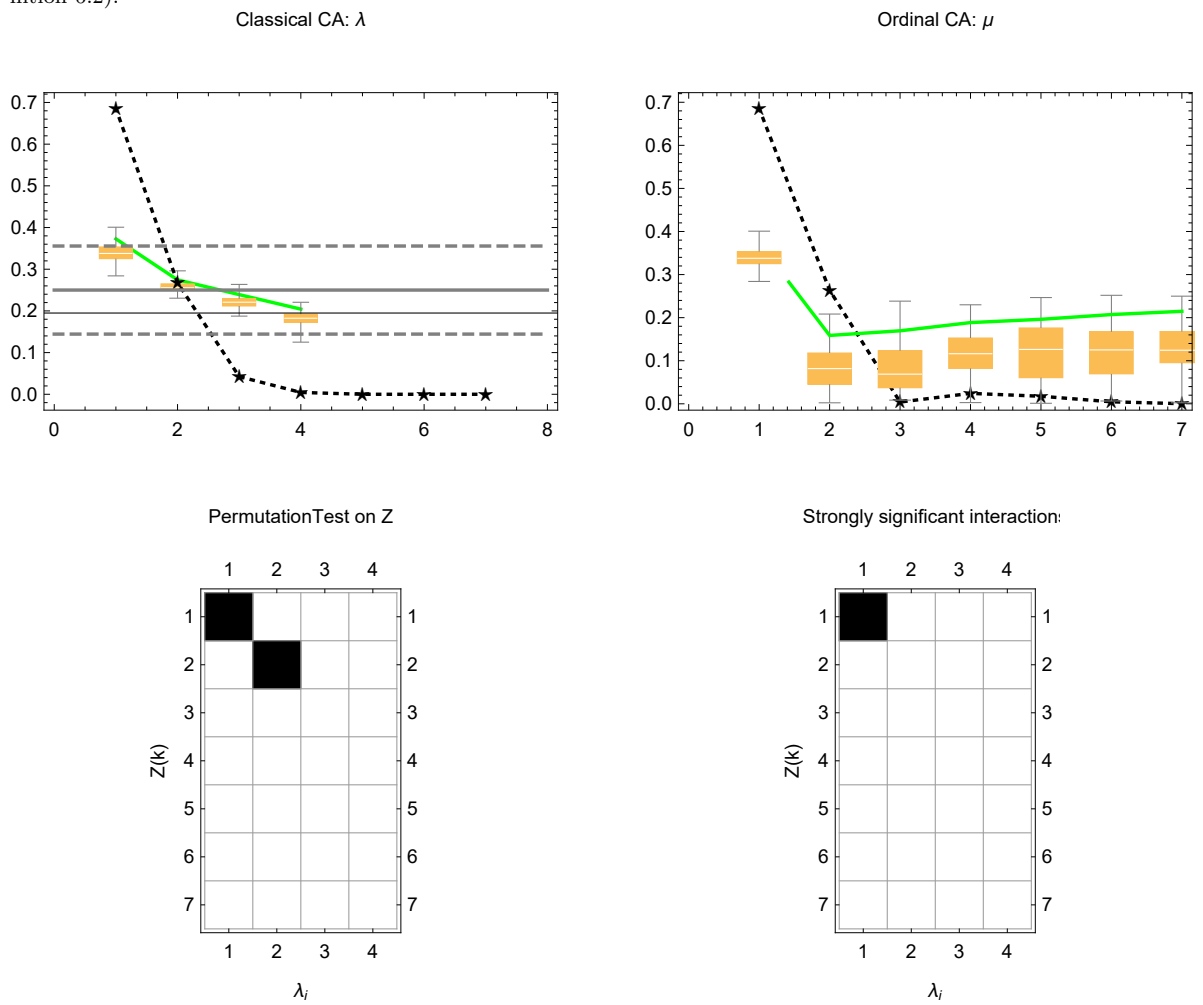
Figure 8. The archaic Chinese vases data. Same structure as Figure 2. Upper plots: statistical significance of eigenvalues and polynomials coordinates. Lower plots, left panel: complete table of significant interactions (in black) issued from the permutation test; right panel (in black): strongly significant interactions (see Definition 6.2).
