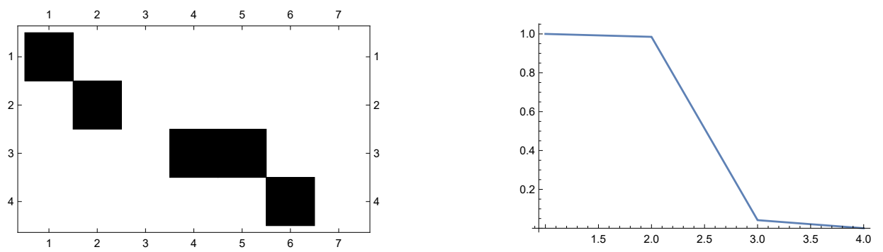
Figure 9. The archaic Chinese vases data: representation of the table of similarities between the sorted factors \pi \odot \varphi_f and the \mathfrak{P}_k . On the left panel, black cells correspond to similarities greater than the fixed threshold (0.1). On the right panel, we plotted the values extracted from the diagonal of this table.
