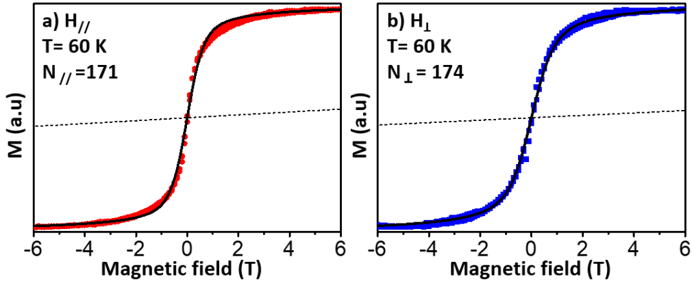
FIG. 6: Magnetization ( M ) of 4 \text{ML}_{\text{Co}} recorded at 60 K at the L_3 Co edge. (a) M as a function of the applied field measured in the H_{\parallel} configuration with \theta = 70^\circ , normalized to its saturation value at 6 T (filled red dots). The solid line is the fit to the data according to Eq. (1) with m_{\text{tot}\parallel} = 1.06 \mu_B/\text{at} and K_{\parallel} = 48 \mu\text{eV}/\text{at} , giving N_{\parallel} = 171 . The dashed line corresponds to the magnetization of an isolated Co atom, given by Eq. (1) with N=1 . (b) the same as (a) in the H_{\perp} configuration with m_{\text{tot}\perp} = 0.98 \mu_B/\text{at} and K_{\perp} = 51 \mu\text{eV}/\text{at} , giving N_{\perp} = 174 . Experimental magnetization M is represented with filled blue squares.
