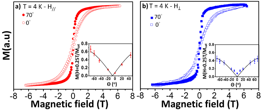
FIG. 4: Magnetization ( M ) of 4 \text{MLCo} recorded at 4 K at the L_3 Co edge. M as a function of the applied field in the (a) H_{//} configuration and (b) H_{\perp} configuration. Magnetization curves are measured at the grazing incidence ( \theta = 70^\circ , filled red dots and filled blue squares) and at the normal incidence ( \theta = 0^\circ , open red dots and open blue squares). The curves have been normalized to their saturation value at 6 T. Insets: angular dependence of the magnetization. Variation in both configurations of the magnetization at 0.25 T normalized to the saturation magnetization at 6 T ( M_{\text{sat}} ) as a function of the incidence angle \theta . The solid lines are fits of the data according to the function a|\sin(\theta - \theta_0)| .
