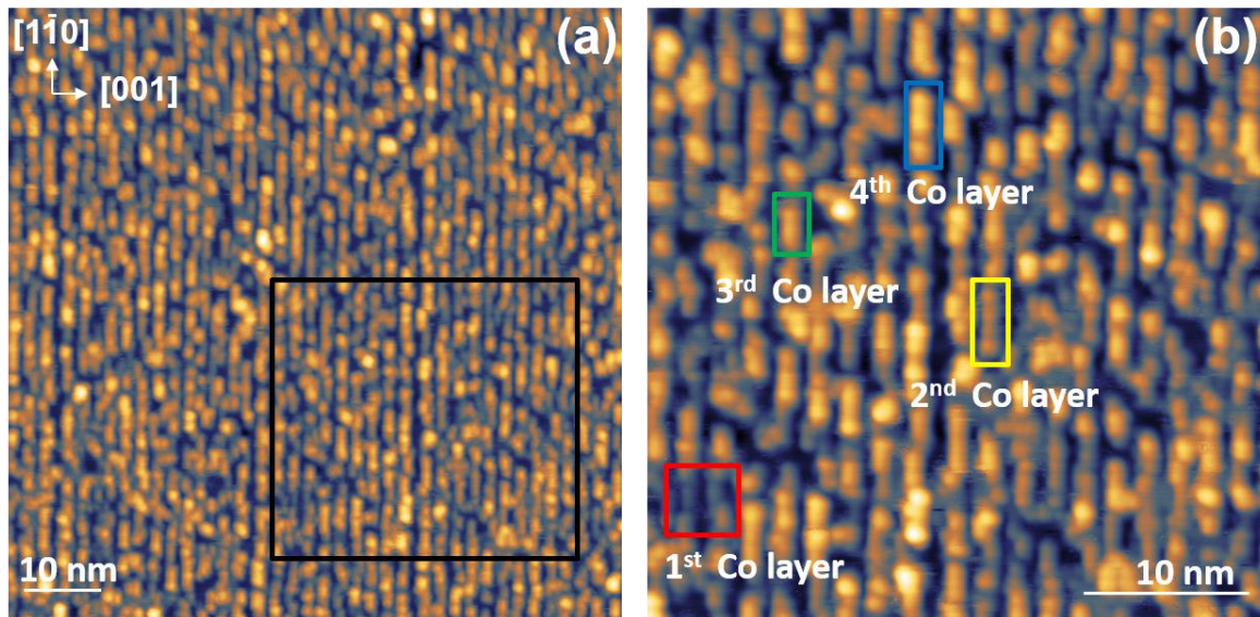
FIG. 2: STM images of an ultrathin film of Co nanolines (coverage \leq 4 ML Co ) after deposition of Co at RT on the 5 \times 2 Si array. (a) 100 nm x 100 nm. (b) Close view (50 nm x 50 nm) of the area indicated in (a) by the black square box. Co nanolines of the different layers are indicated by colored rectangles.
