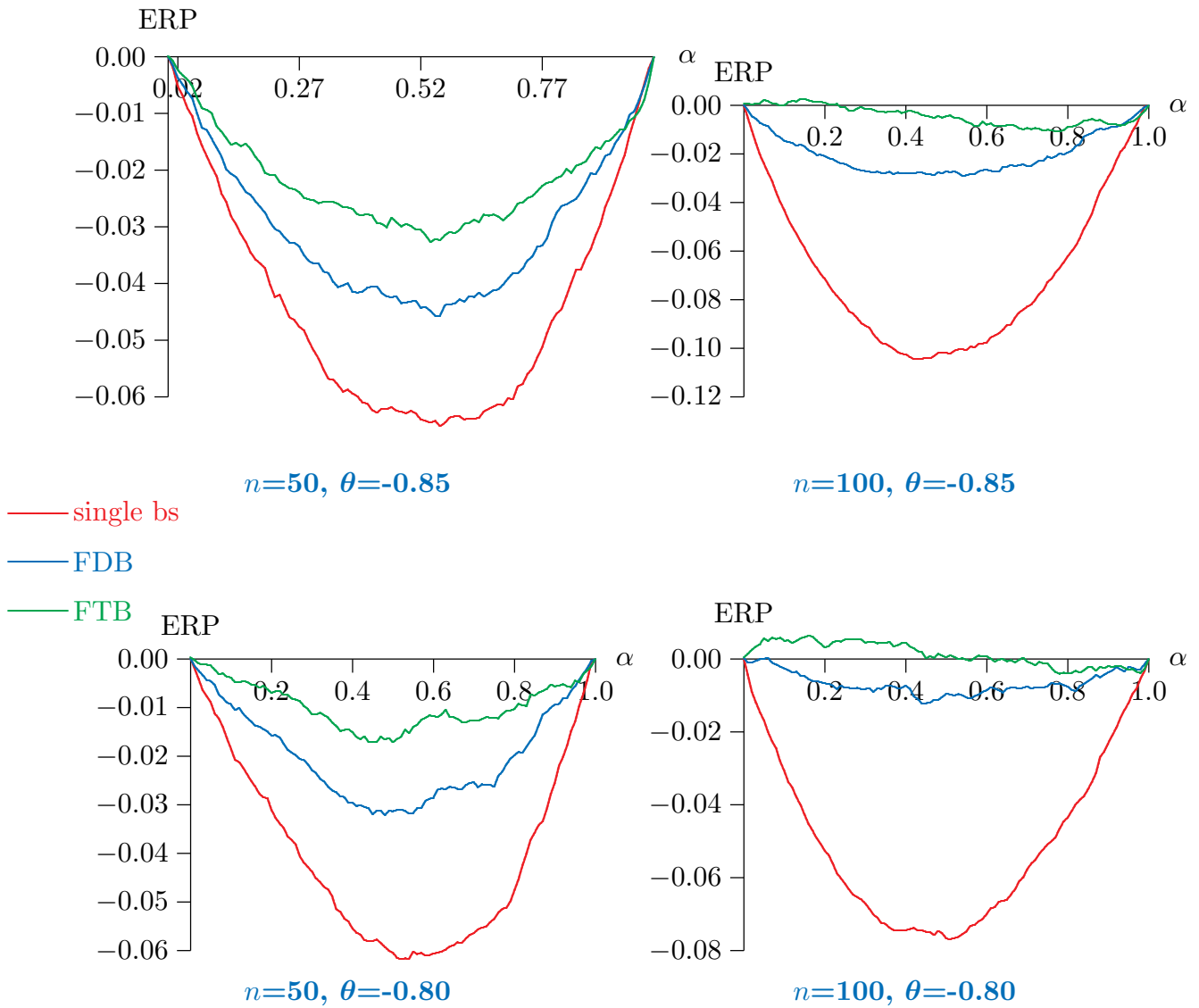
Figure 2: ERPs of unit root test
