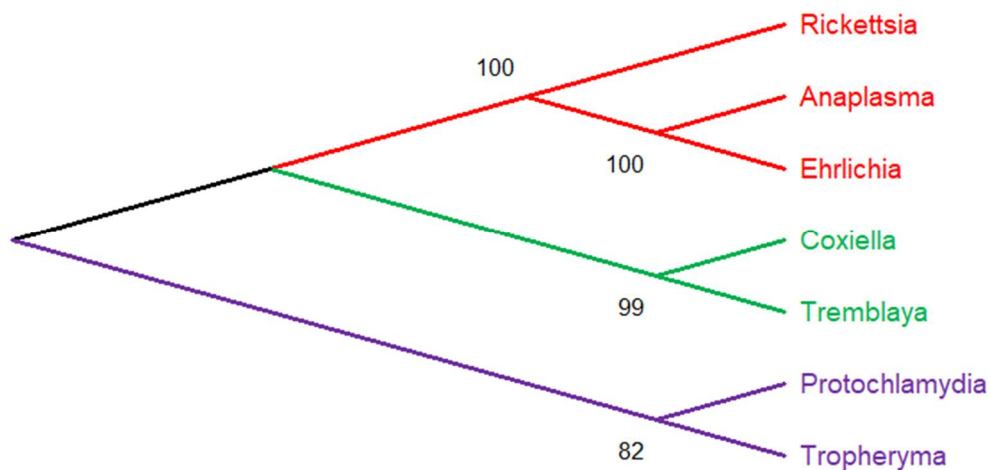
Figure 1. Erroneous phylogenetic relationships between seven obligate intracellular parasitic bacteria. Top: The neighbor-joining tree was generated from 1014 conserved sites in the multiple alignment of their DNA polymerase alpha subunits using the JTT substitution matrix. The protein NCBI identifiers are indicated. In absence of free-living bacterial relatives, the tree erroneously suggests (with a strong statistical support) the existence of 3 separate “parasite families” emerging from 3 distinct evolutionary branches (Alpha, Beta, Gamma). Bottom: Using a different representation, the tree topology (inherent to the tree-building algorithm) can be interpreted as supporting the existence of an ancestral obligate parasite from which all three families of extant parasites derived. The true evolutionary history of these parasitic bacteria is shown in Figure 2.
