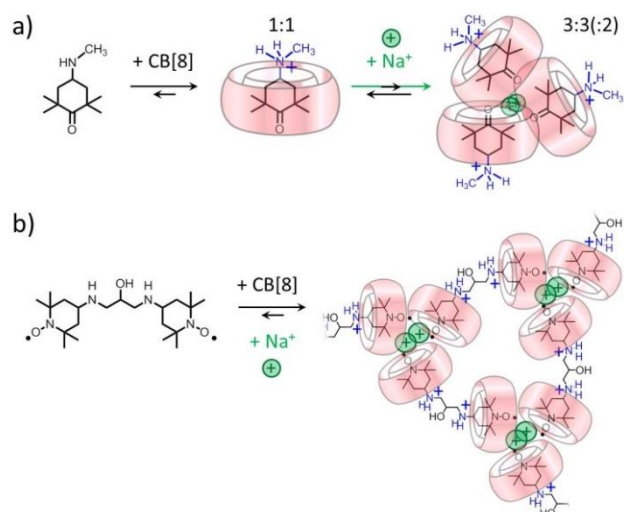
Figure 15. Example of a 1:1 \rightarrow 3:3 equilibrium (a), shifted to the triangular assembly with \text{Na}^+ cations and reticulation (b) by a ditopic guest. [34]
