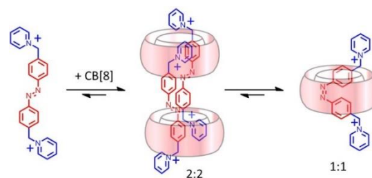
Figure 10. Transient formation of a CB[8]-based 2:2 complex with a switchable, cationic azobenzene derivative.
