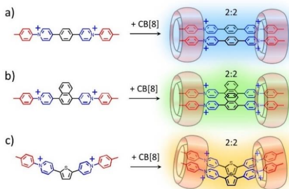
Figure 12. 2:2 complexes of “extended” viologens with CB[8]. The central part of the guest was changed for tuning the photophysical properties of the guest.
