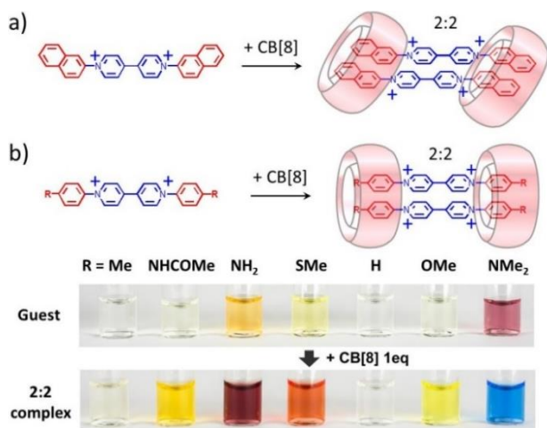
Figure 11. Diaryl-viologens can be relevant guests to form 2:2 complexes with CB[8] as shown by a bisnaphthyl-viologen (a) or bisphenyl-viologens (b) carrying various electron-donating groups. The complexation can be accompanied by dramatic color changes of guest aqueous solutions. Adapted from “G. Wu, M. Olesinska, Y. Wu, D. Matak-Vinkovic and O. A. Scherman, J. Am. Chem. Soc. 2017, 139, 3202” – Published by the American Chemical Society in open access [Creative Commons Attribution (CC-BY license)].
