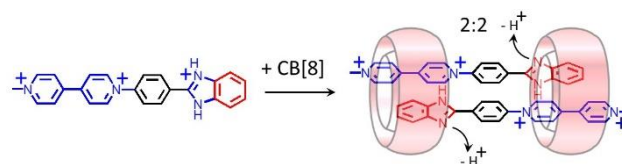
Figure 6. Negative pK_a shift by 2:2 complex formation with CB[8].
