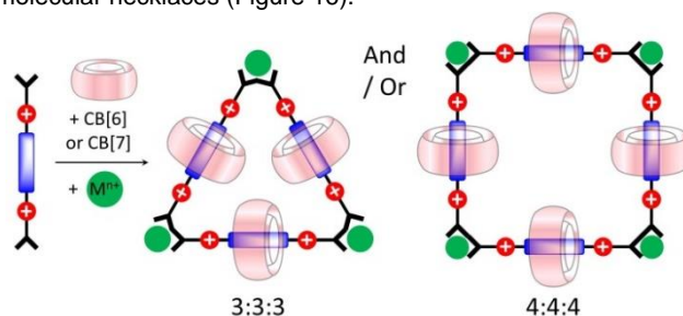
Figure 16. A general approach to get triangular or square molecular necklaces using CBs, the right guests and metal ions.
