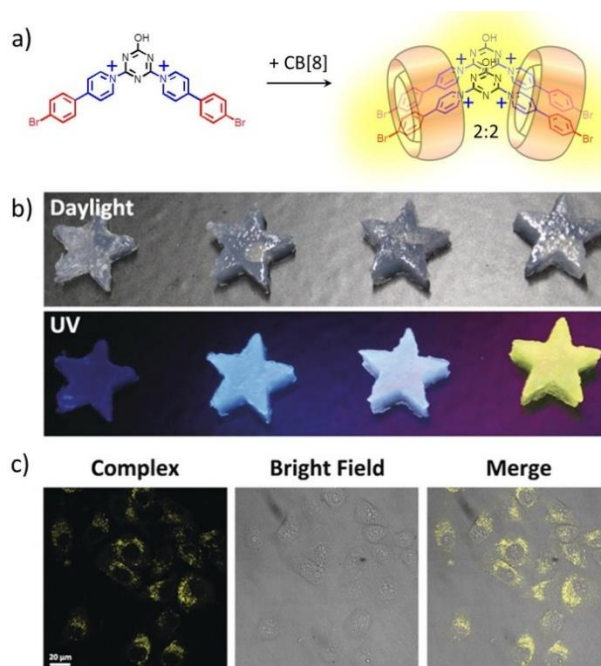
Figure 13. A bis-(aryl-pyridinium)-triazine guest forming an emitting 2:2 complex (a) with CB[8]. Phosphorescent properties are highlighted in panel (b) while fluorescence imaging in cells (c) was also reported. Adapted from “J. Wang, Z. Huang, X. Ma, H. Tian, Angew. Chem. Int. Ed. , 2020, DOI: 10.1002/anie.201914513” – Published by Wiley.
