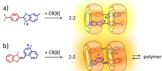
Figure 4. Formation of 2:2 complexes of Thioflavin T (a) and Thiazole Orange (b) after addition of CB[8] in water.
