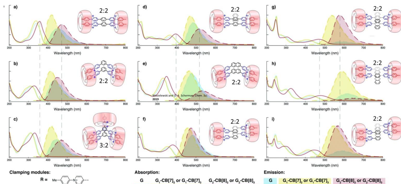
Figure 14. Modular approach of constraining two fluorescent compounds by clamping the periphery of ditopic (two sites of binding) or tritopic (three sites of binding) guests by two or three CB[8]. Absorption and emission spectra of the guests and corresponding 2:2 or 2:3 complexes are shown above highlighting the possible modulation of photophysical properties determined by the structure of the guest. Adapted from "G. Wu, Y. J. Bae, M. Olesińska, D. Antón-García, I. Szabó, E. Rosta, M. R. Wasielewski and O. A. Scherman, Chem. Sci. , 2020, 11, 812" – Published by the Royal Society of Chemistry.
