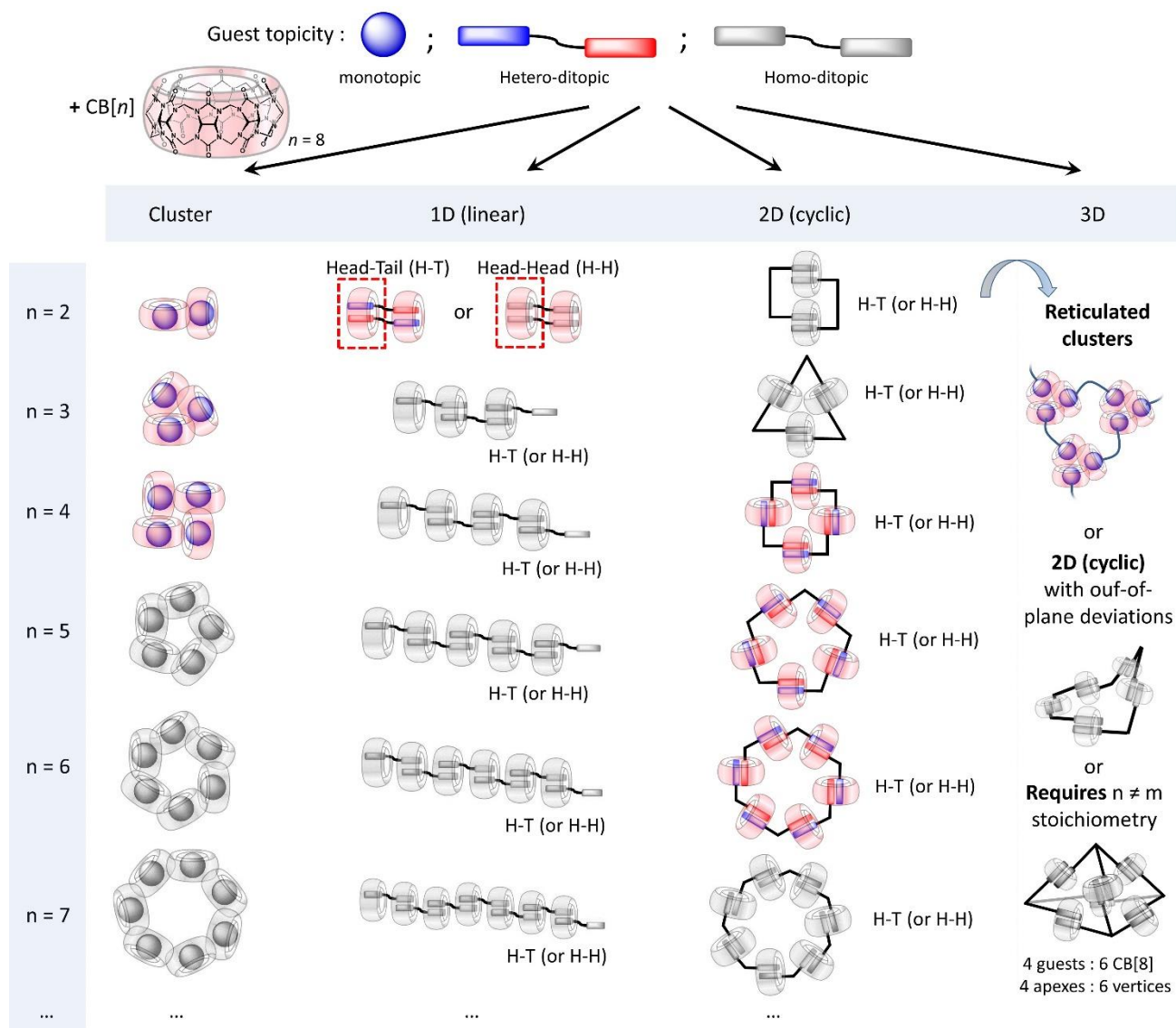
Figure 1. Groups of oligomeric assemblies comprising an identical number “ n ” of cucurbituril hosts and guests (example with CB[8]). Colored structures are described while greyscale assemblies are not reported to the best of our knowledge. Note the group of short-oligomers (linear assemblies), the problem of mismatches for end-groups and the possible advantage upon cyclization. Besides monotopic (one site of binding) guests (cluster column), both hetero-ditopic (two different sites of binding) and homo-ditopic (two identical sites of binding) guests have been used to produce a rapidly growing family of (\text{Host})_n:(\text{Guest})_n superstructures while 3D assemblies remain hard to do.
