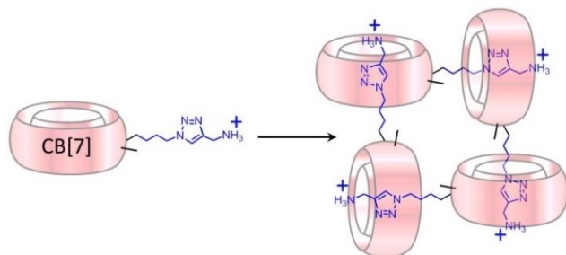
Figure 19. Example of a tetramer of a CB[7] derivative regarded as a covalent analogue of the 4:4 assemblies.
