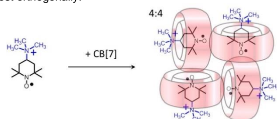
Figure 17. Scheme of the 4:4 CB[7]-nitroxide oligomer.
