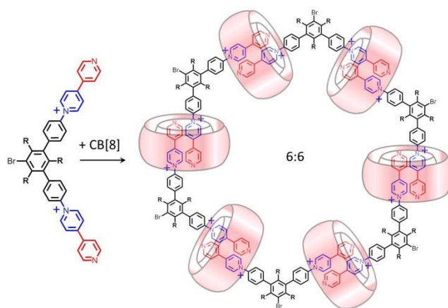
Figure 21. A 6:6 complex based on CB[8] co-sequestration of pyridine-pyridinium blocks, 120° related by a central 1,3-triphenylene core.
