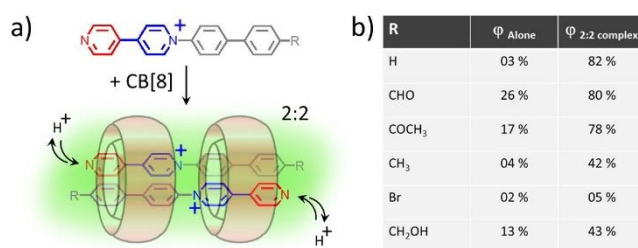
Figure 5. 2:2 complexes of aryl-pyridinium guests and CB[8] (a) with corresponding improvements of fluorescence quantum yields (b).
