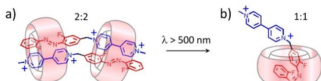
Figure 7. Light-triggered trans-cis isomerization reorganizing 2:2 complexes into 1:1 complexes.
