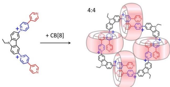
Figure 18. A square 4:4 complex of CB[8] with a dipyrindinium-carbazole guest.
