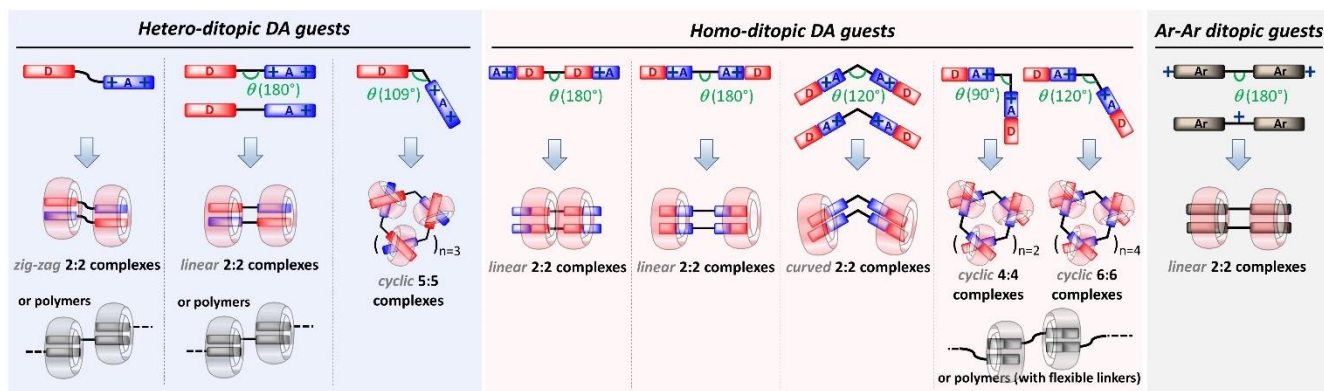
Figure 2. Main ditopic guest molecules affording oligomeric, or polymeric assemblies with CB[8]. The H-H (Head-to-Head) versus H-T (Head-to-Tail) arrangements are important, as flexibility, rigidity, or angles between building-blocks. The number and the place of cationic charges are also important as they are required to improve solubility and binding to CB, and also affect the outcome of the assembly in water. Most discrete oligomers are 2:2 complexes, the variety of which is rapidly increasing, and cyclic oligomers are an emerging class of supramolecular assemblies. (D = donor; A = acceptor). These motifs can tentatively be used as guiding principles to the design of oligomeric cucurbiturils complexes.
