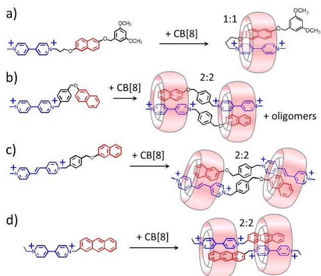
Figure 3. Examples of hetero-ditopic guests leading to 1:1 and "zig-zag" 2:2 complexes upon addition of CB[8].
