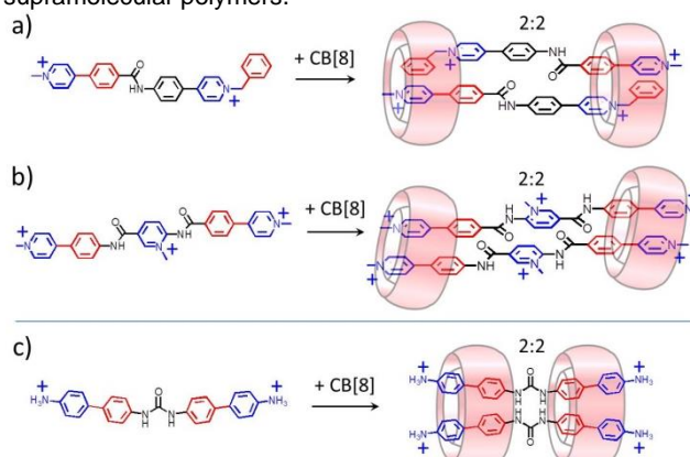
Figure 9. Three types of 2:2 complexes based on asymmetric guest molecules (a and b) and a bis-biphenylammonium-urea (c) with CB[8].
