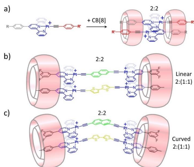
Figure 8. 2:2 complexes (a) based on CB[8] and platinum-terpyridyl complexes (R = 4-tolyl or 3,5-difluorobenzene; R' = H, CH 3 , 4-tolyl). Heteroquaternary 2:2 complexes (b and c) in which the rigid diplatinum guest templated linear ( trans dithiophene) or bent ( cis dithiophene) conformations.
