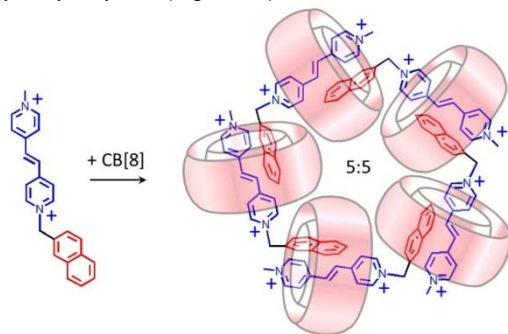
Figure 20. A 5:5 complex of CB[8] and a naphthalene-dipyridiumylethylene guest.
