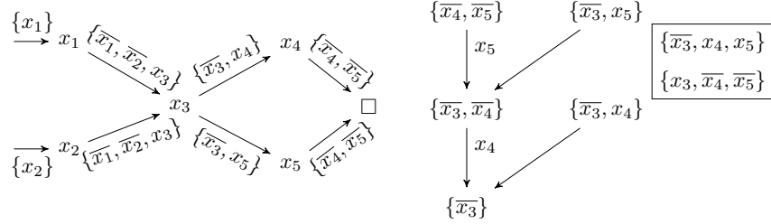
Figure 2: Implication graph corresponding to a propagation sequence of \psi and its transformation by Max-SAT resolution, where compensation clauses for each step are represented in boxes
