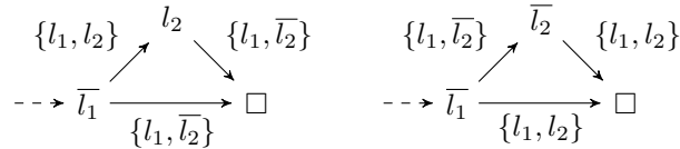
Figure 4: Implication graphs corresponding to the possible propagation sequences for an IS containing the premises of pattern (P1)
