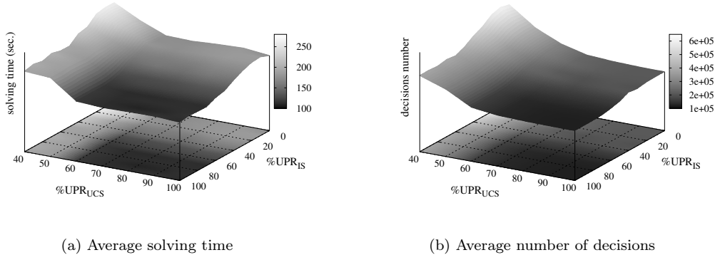
Figure 13: Impact of the minimum percentage of UP-resilience allowed for learning the transformations of ISs and UCSs
