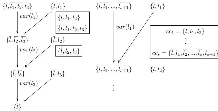
Figure 11: Application of Max-SAT resolution steps on the variables of the non binary clause c by induction on its size ■
