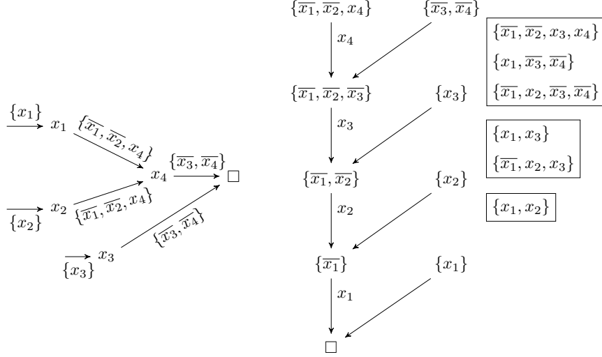
Figure 1: Implication graph corresponding to a propagation sequence of \psi and its transformation by Max-SAT resolution, where compensation clauses for each step are represented in boxes
