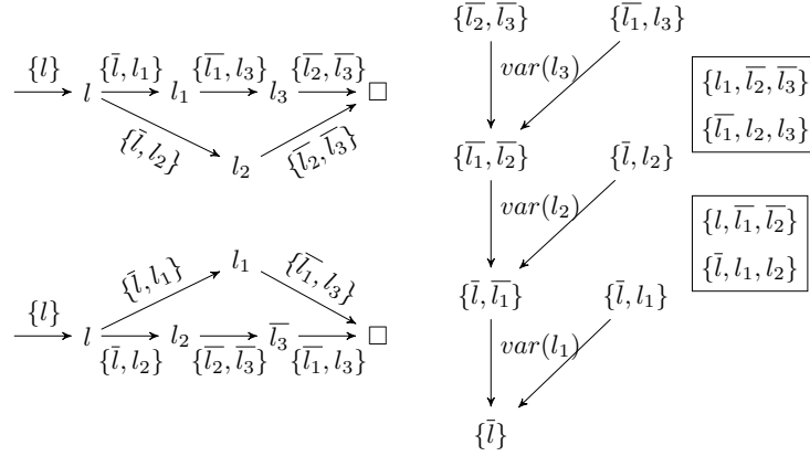
Figure 9: Implication graphs corresponding to the possible propagation sequences of \psi in Example 9 and the application of Max-SAT resolution steps relatively to RPO
