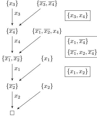
Figure 7: Implication graph corresponding to the Max-SAT resolution transformation of \psi with respect to SIR
