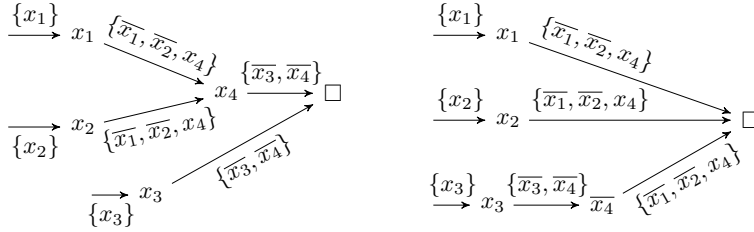
Figure 3: Implication graphs corresponding to the possible propagation sequences of \psi
