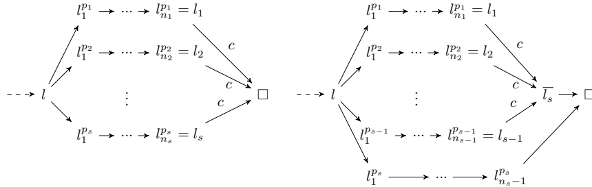
Figure 10: Implication graphs corresponding to the possible propagation sequences for k -UCSs with binary clauses except for the conflict clause
