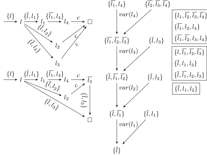
Figure 12: Implication graphs corresponding to the possible propagation sequences of \psi in Example 10 and the application of Max-SAT resolution steps relatively to RPO
