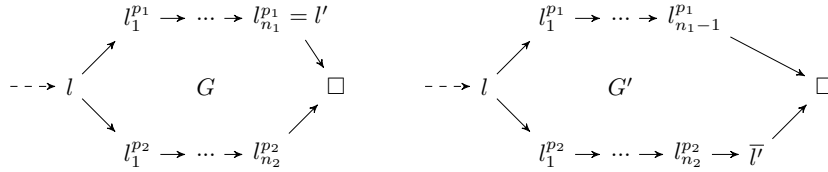
Figure 8: Implication graphs corresponding to the possible propagation sequences for k^b -UCSs.
