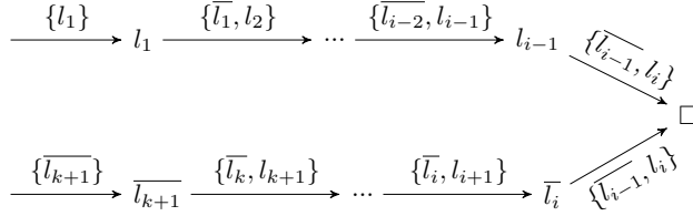
Figure 6: Implication graphs corresponding to the possible propagation sequences for an IS matching the premise of pattern (P3) ■
