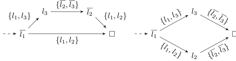
Figure 5: Implication graphs corresponding to the possible propagation sequences for an IS containing the premises of pattern (P_2) ■
