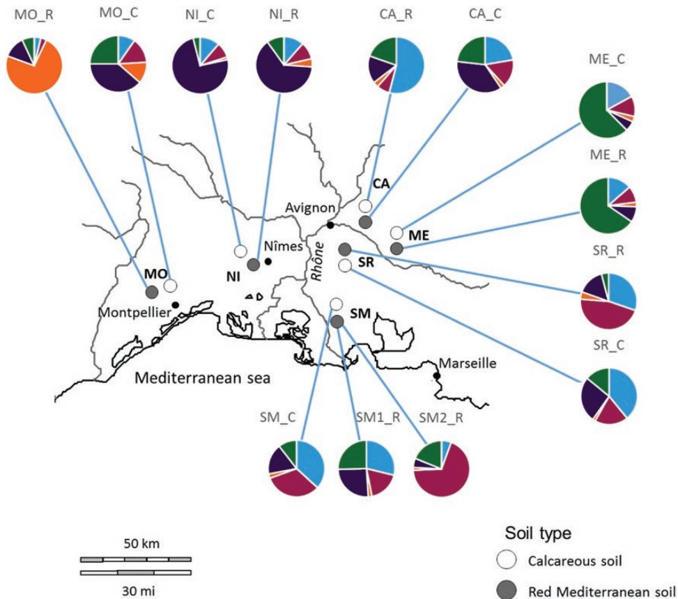
Figure 3. Geographical distribution of the genetic clusters identified by STRUCTURE 2.2 (pie charts) in southern French Brachypodium retusum populations on red Mediterranean and calcareous soil.
