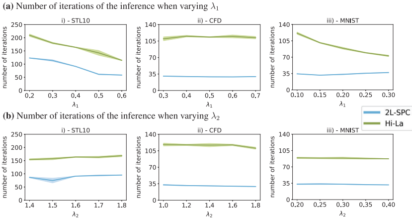
Figure 4: Evolution of the number of iterations needed to reach stability criterion for both 2L-SPC and Hi-La networks on the testing sets of STL-10, CFD, and MNIST databases. We vary the sparsity in the (a) first layer in the top three graphs and sparsity in the (b) second layer in the bottom three graphs. Shaded areas correspond to the mean absolute deviation on seven runs.
