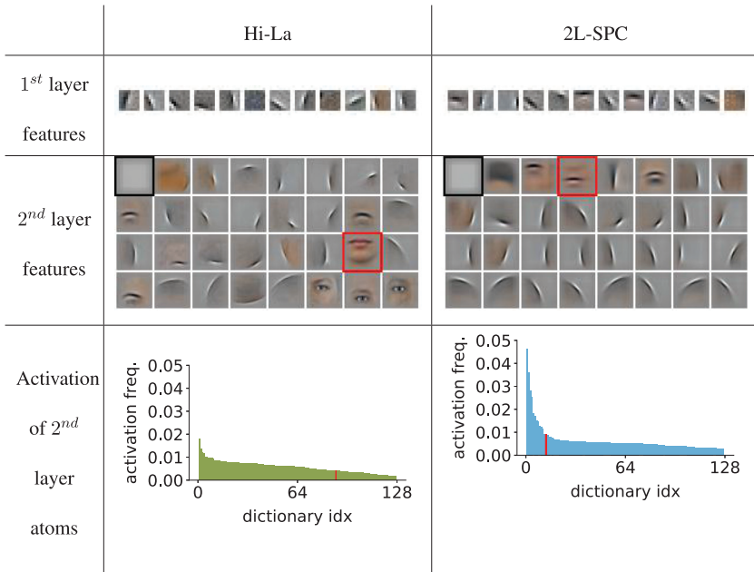
Figure 7: Hi-La and 2L-SPC RFs obtained on the CFD database (with \lambda_1 = 0.3 , \lambda_2 = 1.8 ) and their associated second-layer activation probability histogram. The first- and second-layer RFs are 9 \times 9 px and 33 \times 33 px respectively. For the first-layer RFs, we randomly selected 12 of 64 atoms. For the second-layer RFs, we sampled 32 of 128 atoms and ranked them by their activation probability in descending order. For readability, we removed the most activated filter (RF framed in black) in 2L-SPC and the Hi-La second-layer activation histogram. The activation probabilities of the RFs framed in red are shown as a red bar in the corresponding histogram.
