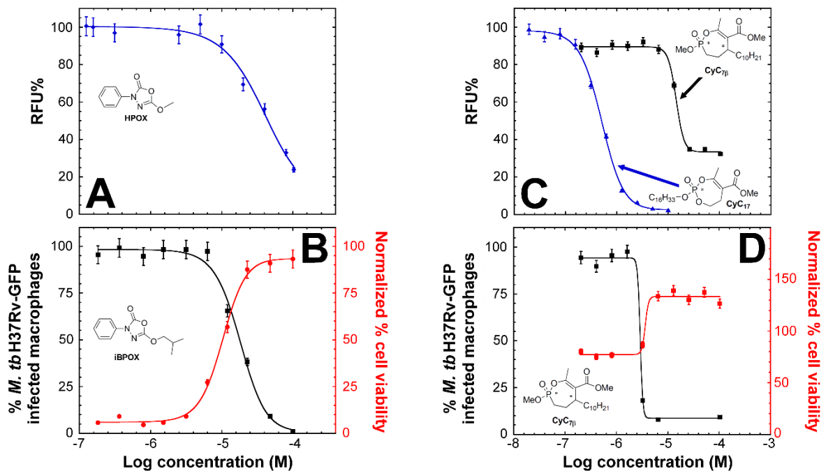
306 307 Figure 4. (A-C) Activity of HPOX , CyC7β & CyC17 against GFP-labelled M. tb H37Rv 308 replicating in culture medium expressed as normalized relative fluorescence units (RFU%). (B- 309 D) Activity of iBPOX and CyC7β against M. tb H37Rv-GFP replicating inside Raw264.7 310 macrophages. Adapted from [54, 61]. 311
