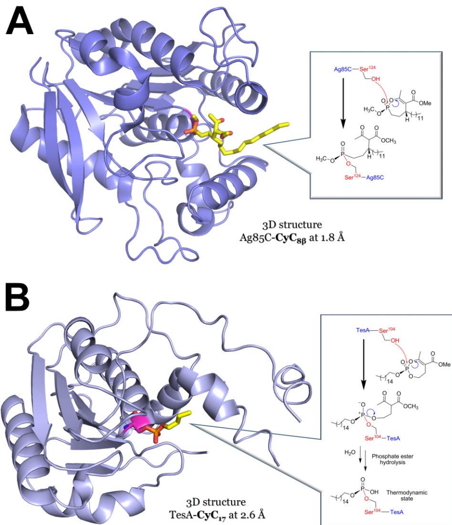
Figure 6. Crystal structures of (A) Ag85C in complex with CyC 8β (PDB ID: 5OCJ; 1.8Å resolution) [78] and (B) TesA in complex with CyC 17 (PDB ID: 6FVJ; 2.6Å resolution) [79]. The mechanism of action of the phosphonate ( CyC 8β ) and the phosphate ( CyC 17 ) analog based on mass spectrometry analyses are illustrated in inset. Each inhibitor is in stick representation, and the catalytic Serine residue is colored in magenta. Structures were redrawn as ribbon representations from their respective modified PDB IDs, with PyMOL Molecular Graphics System (Schrödinger, LLC).
