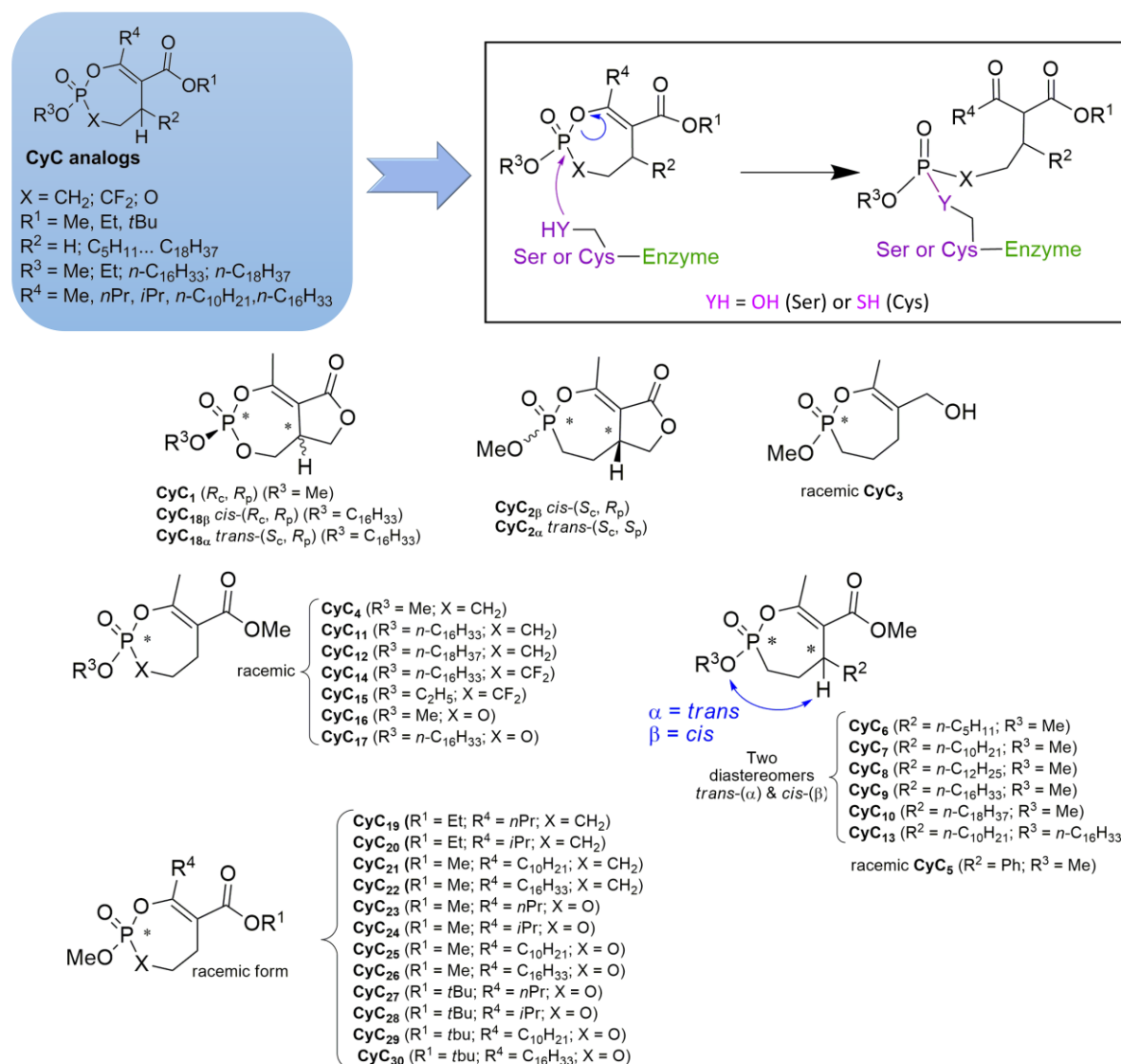
Figure 3. Chemical structure of Cyclipostins & Cyclophostin analogs (CyC), as well as their mechanism of action on (Ser/Cys)-based enzymes in inset. For a review on the CyC synthesis, please refer to [50].
