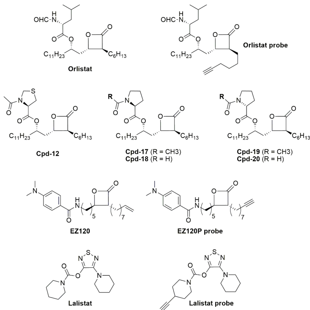
Scheme 1. Chemical structures of Orlistat & Orlistat probe [27], and related \beta -lactones Cpd-12 , Cpd-17-20 [26], EZ120 & EZ120P probe [34]; as well as the human lysosomal acid lipase inhibitor Lalistat and its corresponding alkyne-modified probe [33].
