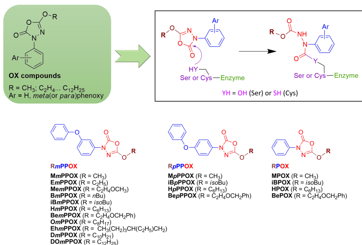
Figure 1. Chemical structure of Oxadiazolone-core derivatives ( OX ) as well as their mechanism of action on (Ser/Cys)-based enzymes in inset.
