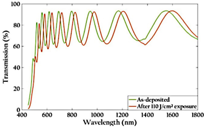
Fig. 1 – Evolution of the spectral dependence of the transmission of a 990 nm thick As_2S_3 layer (green: as deposited layer and red: layer after exposure to a 20 mW LED at 470 nm).
