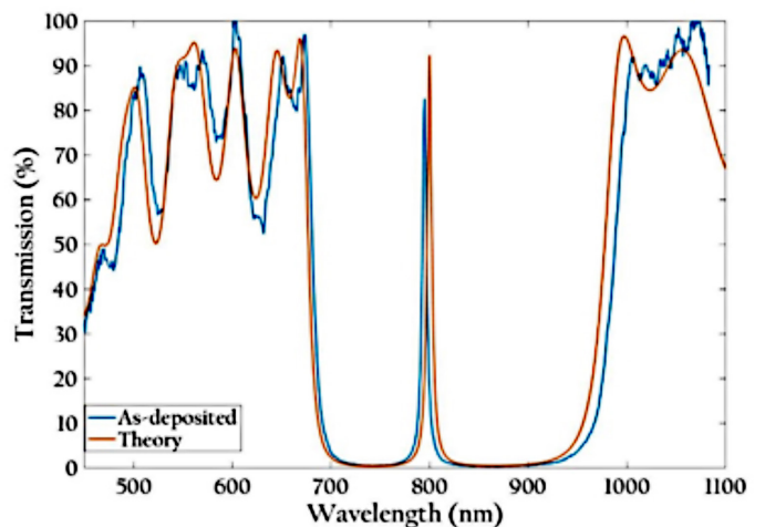
Fig. 3 – Spectral dependence of the transmission of a (HL)^4 / 4 \text{ ChG} / (LH)^4 Fabry Perot filter. Theoretical filter: red curve, experimental filter: blue curve.
