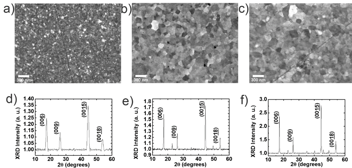
Figure 1. a-c) SEM images obtained in backscattered mode for the a) 10 nm b) 30 nm and c) 50 nm Sb 2 Te 3 layers. d-f) Corresponding XRD diagrams ( \lambda = 0.15418 nm) for the d) 10 nm e) 30 nm f) 50 nm samples.
