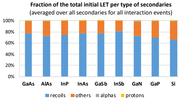
Figure 12. Fraction of the total initial LET deposited per type of secondaries for all interaction events in the bulk of the studied III-V semiconductors.
