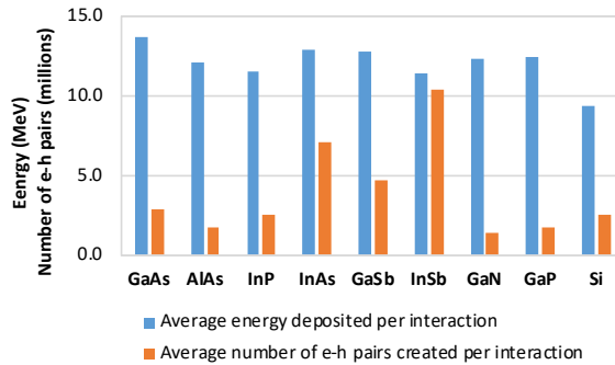
Figure 9. Deposited energy per interaction (mean value estimated from all events) and corresponding amounts of e-h pairs created in the different III-V material targets. Values have been evaluated considering for each material the e-h pair creation energy given in Table I. Typical values for silicon are also indicated for reference.
