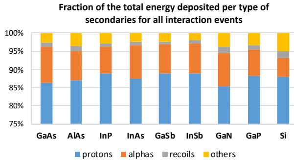
Figure 11. Fraction of the total energy deposited per type of secondaries for all interaction events in the bulk of the studied III-V semiconductors.
