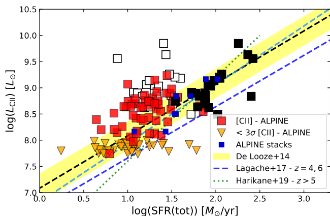
Fig. 2. [C II] as a function of UV or UV+IR-derived SFR for the z \sim 4.5 ALPINE sources. Squares show the [C II] detections, orange triangles the 3\sigma upper limits. Black squares show galaxies with continuum detection (black filled squares show \text{SFR}(\text{UV}) + \text{SFR}(\text{IR}) , empty squares the \text{SFR}(\text{UV}) of the same sources); red squares shows the \text{SFR}(\text{UV}) for the other (non-continuum-detected) ALPINE sources. Blue circles show the results from stacks of ALPINE sources in four bins of L([\text{CII}]) and two redshift bins, adapted from Bethermin et al. (2020). The observations are compared to the [C II]–SFR relations of local galaxies determined by De Looze et al. (2014) adjusted to the Chabrier IMF by reducing the SFR by a factor of 1.06 (black dashed line), shown by the yellow band with a total width corresponding to 2\sigma . The green dotted line shows the relation fitted to observations of z \sim 5 - 9 galaxies by Harikane et al. (2019). The fits from the models of Lagache et al. (2018) for redshifts spanning the range of the observations are shown by the two blue dashed lines.
