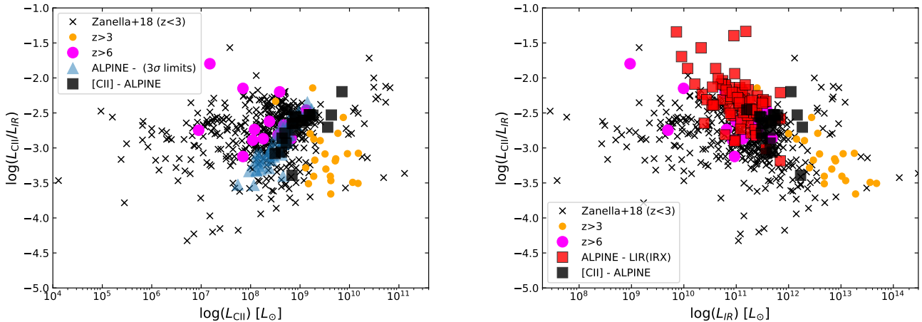
Fig. 8. L([CII])/L_{IR} versus L([CII]) (left panel) and L_{IR} (right) for the ALPINE sources and comparison samples where the [C II] line is detected. For the z > 6 sources, taken from the Matthee et al. (2019) sample, we adopt T_d = 45 K for the detections and L_{IR} upper limits. For galaxies not detected in the dust-continuum, we show their L([CII])/L_{IR} 3\sigma lower limit in the left panel as triangles. In the right panel, the L_{IR} limits of the ALPINE sources have been replaced by the L_{IR} values computed from the IRX- \beta relation, where possible.
