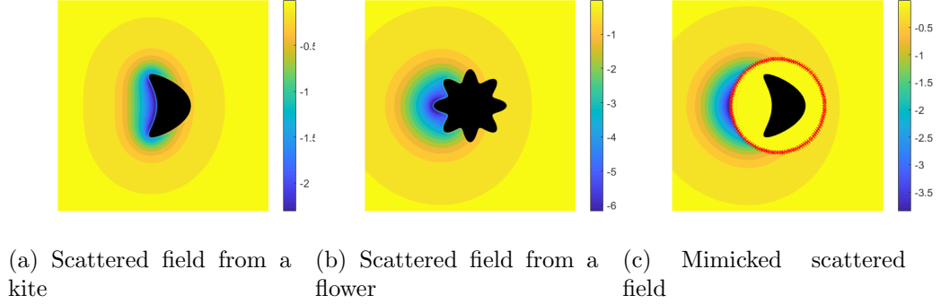
FIGURE 12. Numerical example of the object mimicking problem with a “kite” and “flower” object, both with homogenous Dirichlet boundary conditions. A snapshot the scattered field from the original object at time t = 0.05s appears in (a). In (c), the scattered field from the original object is made to appear as the scattered field from the object in (b) from the perspective of thermal measurements outside of the cloaking region \bar{\Omega} .
