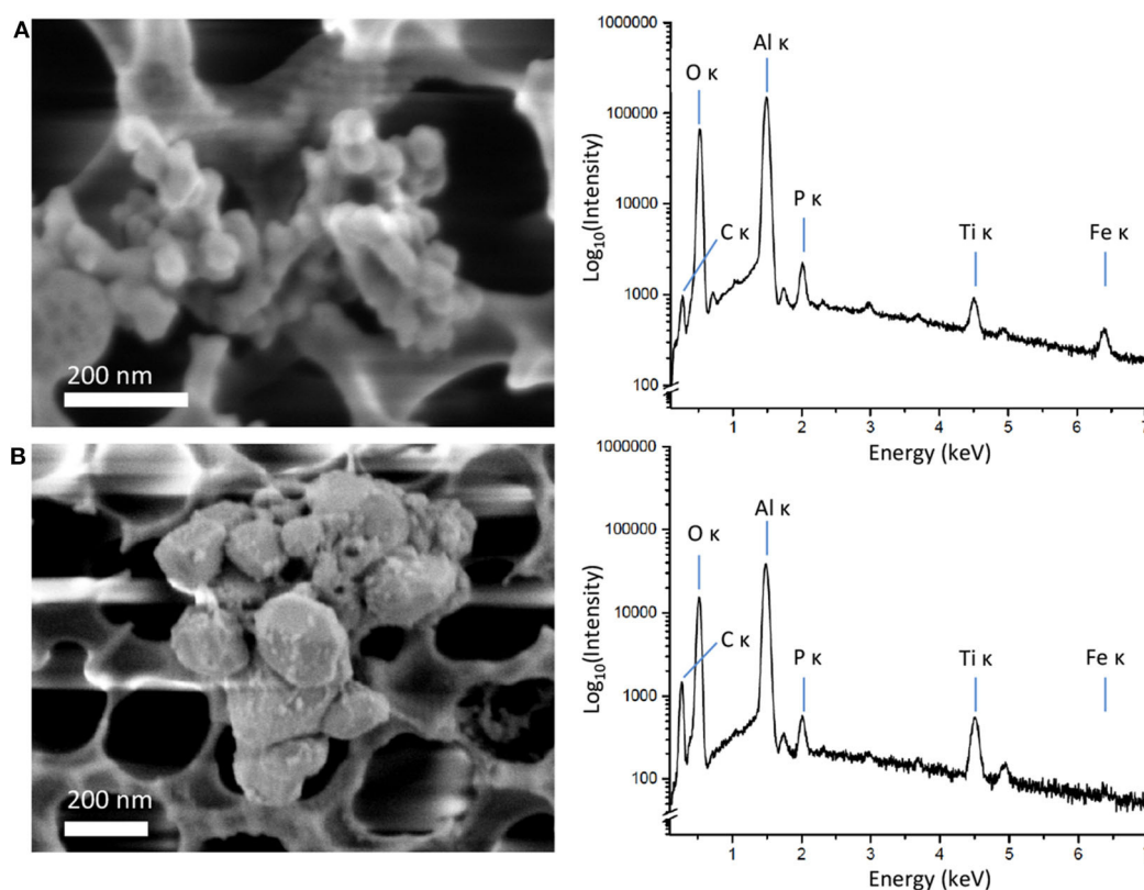
FIGURE 6 | SEM images (left) and corresponding EDS spectra (right) of particles recovered on 0.20 \mu\text{m} filters from (A) Industrial Effluent and (B) WWTP in October 2017. Some charging features present in SEM images as a result of no coating being applied to samples.
