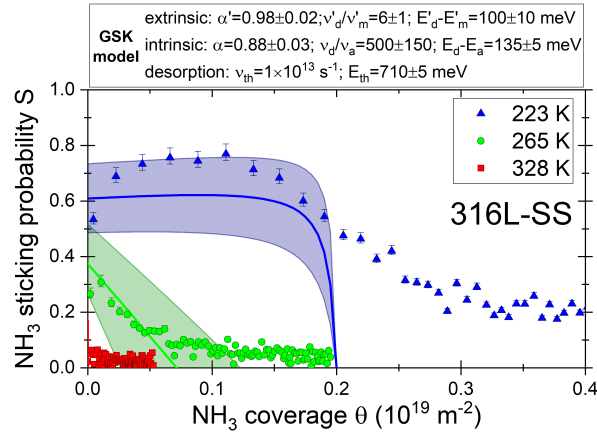
Figure 6: Sticking probability of \text{NH}_3 as a function of ammonia coverage on 316L stainless steel. The kinetic energy of \text{NH}_3 is 55 meV. The curves are a fit to the data employing the GSK precursors-mediated model (Equation 15) presented in the discussion section 4.2 with a saturation (monolayer) coverage of 0.2 \times 10^{19} \text{ m}^{-2} .
