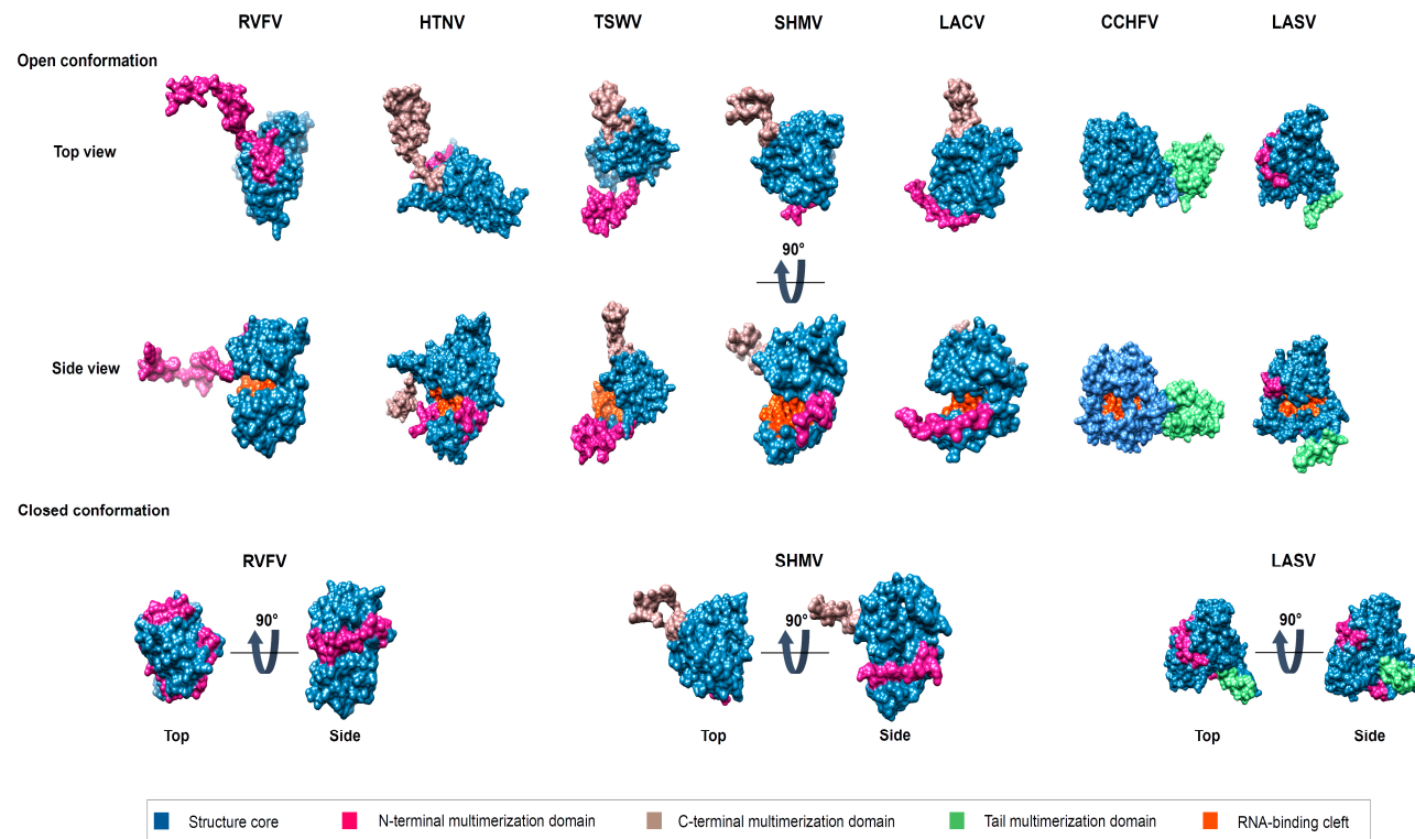
Figure 5. Structural comparison of known Bunyavirales NP. Surface representation of the different structures of representative Bunyavirales from left to right Phenuiviridae (RVFV, open conformation PDB: 3OUO /Closed conformation PDB: 3LYF), Hantaviridae (HTNV, PDB: 5FSG), Tospoviridae (TSWV, PDB: 5IP1), Peribunyaviridae (SHMV, open conformation PDB: 4DIX /Closed conformation PDB: 4DIU, LACV PDB: 4BHH), Nairoviridae (CCHFV, PDB: 4AQF) and, Arenaviridae (LASV core domain, open conformation PDB: 3T5Q /Closed conformation from PDB: 3MWP). Highlighted are the 3 important parts of the NP core in blue, multimerization arms N-terminal in pink, central in green, and the C-terminal in kaki.
