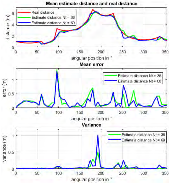
Figure 7: Comparison between real distances and the distances obtained at the velocity \Omega_r = 907^\circ/\text{s} . Red : true distance. Green: N_t = 36 . Blue: N_t = 60 .
