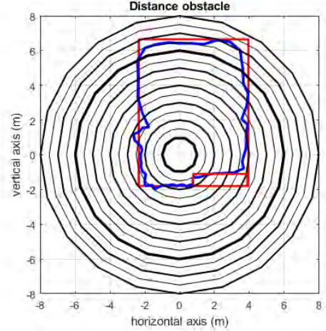
Figure 6: Distance estimated using the proposed method. Bench test is placed inside the central circle. Thick circles are spaced one meter apart, and distance between thick and thin circle correspond to 0.5m. Red : true distance. Blue : N_t = 60 .
