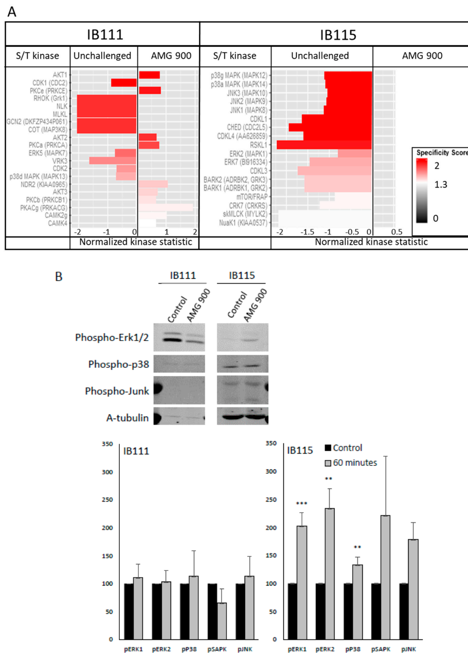
Figure 7. AMG 900 inhibits MAPK activity and modulates phosphorylation in sensitive cell line. (A) Variation of serine/threonine kinomic activity in resistant IB111 and sensitive IB115 with AMG 900 treatment. Cells were treated with IC 50 of AMG 900 for one hour before protein extraction and analysis on PamChip. Kinases activities are compared between unchallenged and AMG 900-treated cells. Peptides phosphorylation leads to a serine/threonine kinases list presenting variation between both conditions. Graphic represent IB111 kinase activity in unchallenged (left) and AMG 900 treated-cell (right), intense red color correspond to high specificity score compare to white color. (B) Differential phosphorylation of MAPK in IB111 and IB115 cell lines, treated or not with AMG 900. Cells were treated with IC 50 of AMG 900 for one hour before protein extraction and analysis by western-blot. Histograms are mean values of triplicate +/-SEM. (**: p < 0.01 ; ***: p < 0.001 ). More details of western blot, please view at the supplementary materials.
