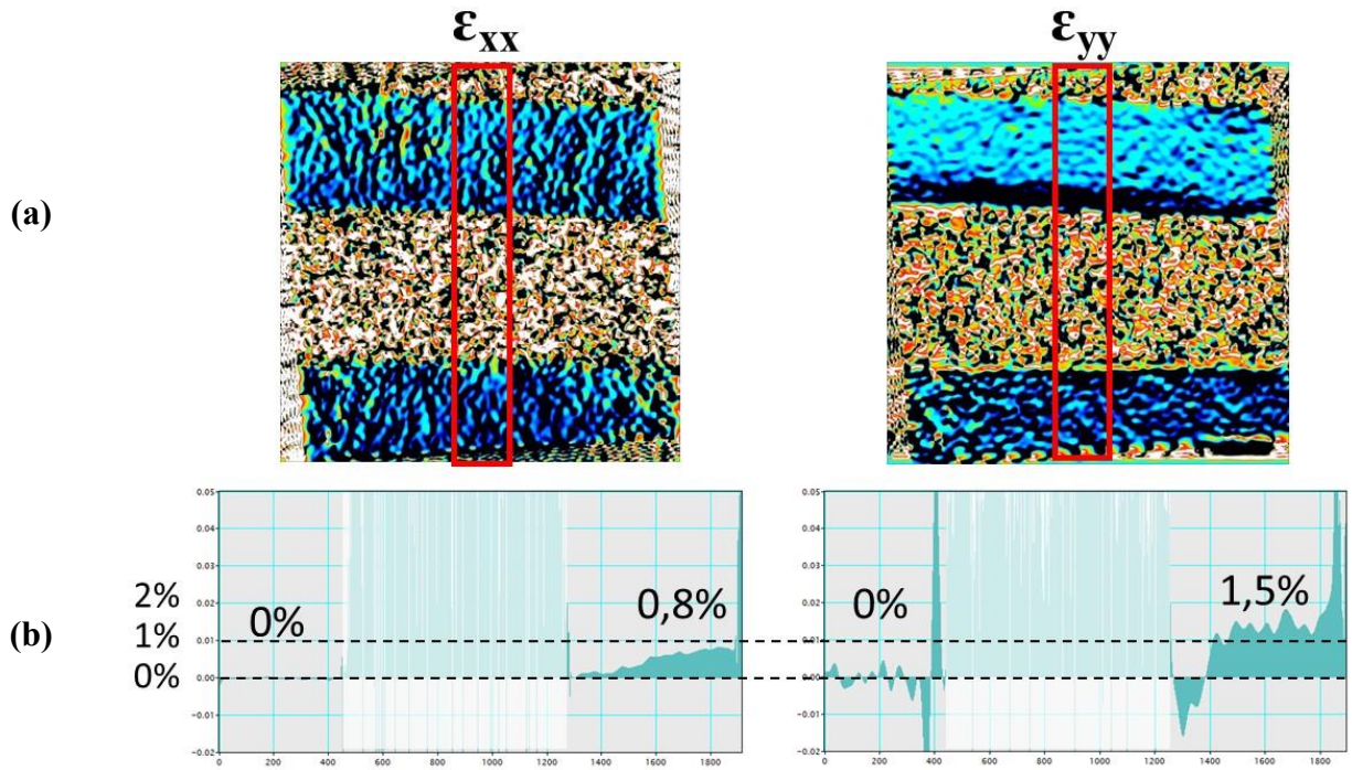
Figure 6: (a) Color scale map of c -planes ( \epsilon_{yy} ) and a -planes ( \epsilon_{xx} ); (b) Distribution of strain integrated on areas pointed by the red squares in (a).
