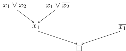
Fig. 5. Regular tree resolution refutation after minimization
