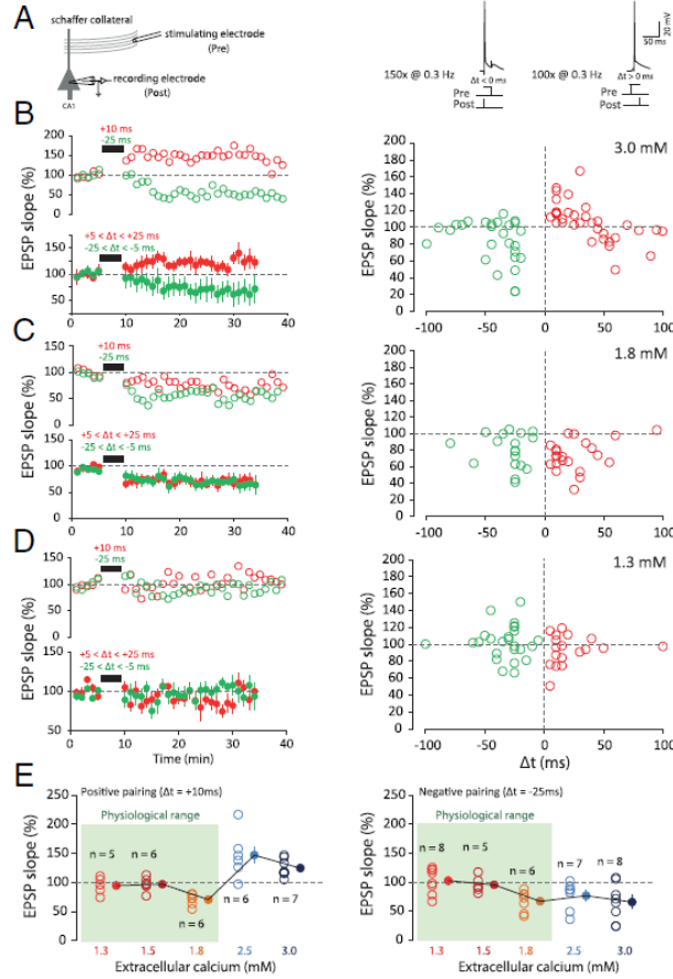
Fig. 2. STDP under various external calcium concentrations. (A) t-LTP and t-LTD are induced at low frequency (0.3 Hz). The pre-post protocol is repeated 100 times, while the post-pre protocol is repeated 150 times. The action potential is induced by the injection of a depolarizing current into a CA1 neuron recorded in a whole-cell configuration. The EPSP is evoked by a stimulation electrode placed in the Schaffer collaterals. The delay ( \Delta t ) is varied according to the experiments. (B) In 3 mM extracellular calcium, a prepost protocol (positive delays; +5 < \Delta t < +25 ms; red) leads to t-LTP and a post-pre (negative delays; -25 < \Delta t < -5 ms; green) protocol leads to t-LTD. Note the presence of a second t-LTD window at around +40/+60 ms. To facilitate comparison between the data, the duration of the negative pairing has been set to that of the positive pairing. (C) In 1.8 mM extracellular calcium, both pre-post protocols ( +5 < \Delta t < +25 ms; red) and post-pre protocols ( -25 < \Delta t < -5 ms; green) lead to t-LTD. The t-LTP window is absent under these conditions. (D) In 1.3 mM extracellular calcium, on average, no plasticity is induced regardless of the delay. The t-LTP and t-LTD window are missing under these conditions. (E, Left) Synaptic changes for a pre-post protocol at +10 ms. No plasticity is induced for calcium concentrations of 1.3 and 1.5 mM. For 1.8 mM calcium, t-LTD is induced, while for 2.5, and 3 mM calcium, t-LTP is induced. (E, Right) Synaptic changes for a post-pre protocol at -25 ms. No plasticity is induced in 1.3 and 1.5 mM calcium. For 1.8, 2.5, and 3 mM calcium, t-LTD is induced. Note the difference between the results in the range of physiological calcium concentration (green squares) and the results in nonphysiological calcium concentration.
