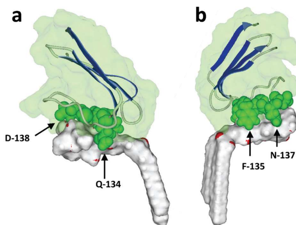
Figure 6. Molecular complex between the NTD of SARS-CoV-2 S protein and a single GM1 ganglioside:
