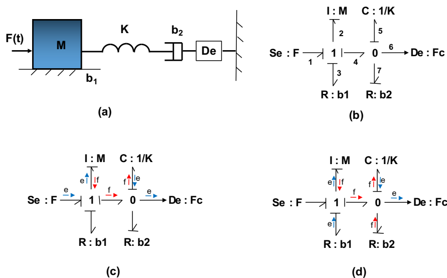
Figure 3. Illustration of an example of the causal paths following from an input to an output: (a) example of the mechanical system, (b) its corresponding BG model, (c,d) causal paths.
