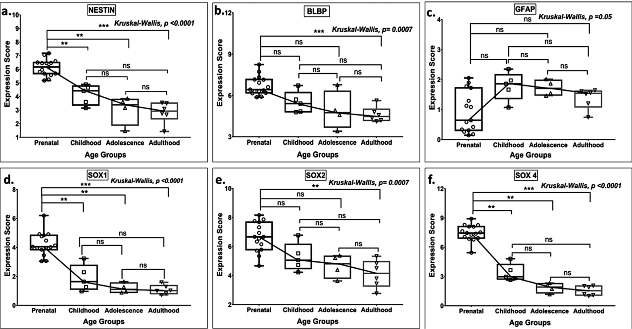
Fig. 1. Box plot presentation (median with minimum and maximum bars showing all data points) of Neurogenesis Stage 1 - Neural stem cell markers ( NESTIN , BLBP , GFAP , SOX1 , SOX2 , SOX4 ), gene expression scores in log2 of RPKM(reads per kilobase of exon model per million mapped reads).Statistical comparisons were made using the Kruskal-Wallis test followed by a post hoc Mann Whitney U test and FDR correction. Adjusted p-values for MWU comparisons represented by, **** \leq 0.0001 , *** \leq 0.001 , ** \leq 0.01 , and ns for non-significant.
