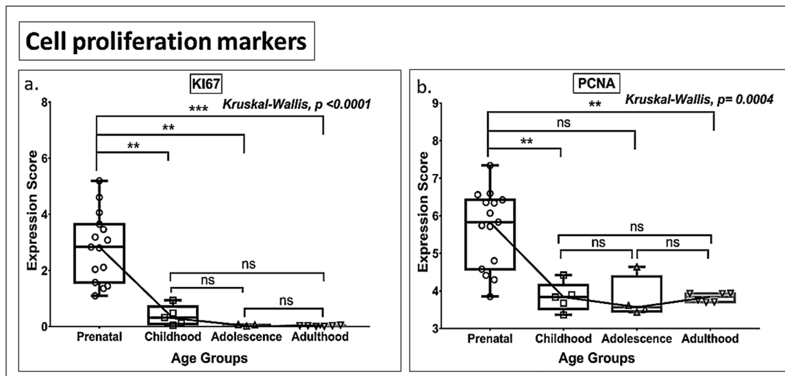
Fig. 9. Box plot presentation (median with minimum and maximum bars showing all data points) of Cell proliferation markers ( KI67 , PCNA ), gene expression scores in log2 of RPKM (reads per kilobase of exon model per million mapped reads). Statistical comparisons were made using the Kruskal-Wallis test followed by a post hoc Mann Whitney U test and FDR correction. Adjusted p -values for MWU comparisons represented by, **** \leq 0.0001 , *** \leq 0.001 , ** \leq 0.01 , and ns for non-significant.
