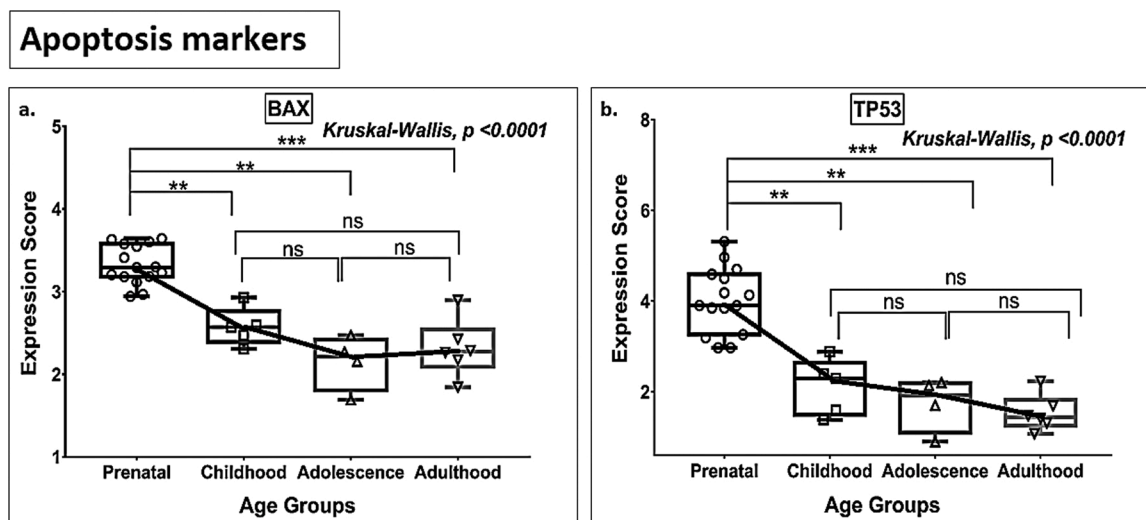
Fig. 10. Box plot presentation (median with minimum and maximum bars showing all data points) of Apoptosis markers ( BAX , TP53 ), gene expression scores in log2 of RPKM (reads per kilobase of exon model per million mapped reads). Statistical comparisons were made using the Kruskal-Wallis test followed by a post hoc Mann Whitney U test and FDR correction. Adjusted p -values for MWU comparisons represented by, **** \leq 0.0001 , *** \leq 0.001 , ** \leq 0.01 , and ns for non-significant.
