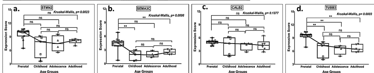
Fig. 4. Box plot presentation (median with minimum and maximum bars showing all data points) of Neurogenesis Stage 4 - Axonal and dendritic targeting/Early maturation markers ( STMN2 , SEMA3C , CALB2 , TUBB3 ), gene expression scores in log2 of RPKM (reads per kilobase of exon model per million mapped reads). Statistical comparisons were made using the Kruskal-Wallis test followed by a post hoc Mann Whitney U test and FDR correction. Adjusted p-values for MWU comparisons represented by, **** \leq 0.0001 , *** \leq 0.001 , ** \leq 0.01 , and ns for non-significant.
