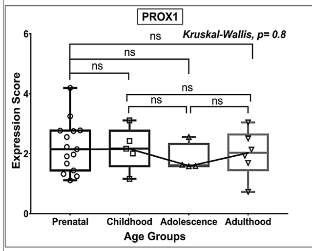
Fig. 6. Box plot presentation (median with minimum and maximum bars showing all data points) of the pan-neuronal lineage marker PROX1 , gene expression score in log2 of RPKM (reads per kilobase of exon model per million mapped reads). Statistical comparisons were made using the Kruskal-Wallis test followed by a post hoc Mann Whitney U test and FDR correction. Adjusted p-values for MWU comparisons represented by, **** \leq 0.0001 , *** \leq 0.001 , ** \leq 0.01 , and ns for non-significant.
