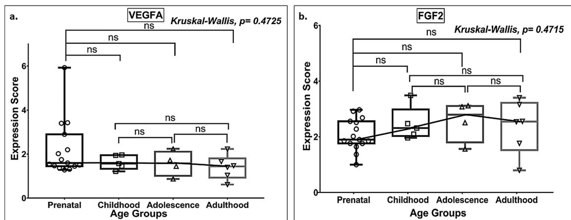
Fig. 8. Box plot presentation (median with minimum and maximum bars showing all data points) of Vasculogenesis markers ( VEGFA , FGF2 ), gene expression scores in log2 of RPKM (reads per kilobase of exon model per million mapped reads). Statistical comparisons were made using the Kruskal-Wallis test followed by a post hoc Mann Whitney U test and FDR correction. Adjusted p-values for MWU comparisons represented by, **** \leq 0.0001 , *** \leq 0.001 , ** \leq 0.01 , and ns for non-significant.
