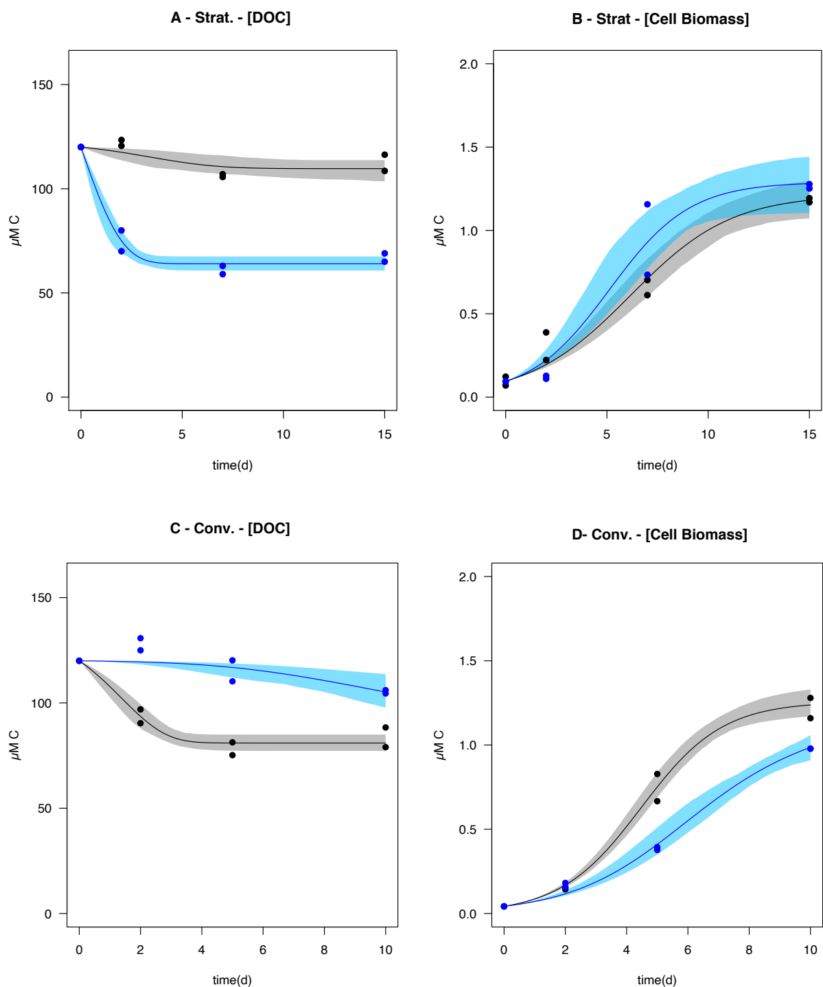
Figure 2. Changes in DOC concentrations (A, C), cell biomass concentrations (B, D) in \mu\text{M C} over time (in days) during stratified period (Strat.) and deep-water mass convection period (Conv.). Blue and black dots are observations respectively for HP and DEC incubations. Blue and black lines are predicted data by model and blue and grey variability bands are 95% confident intervals, respectively for HP and DEC incubations.
