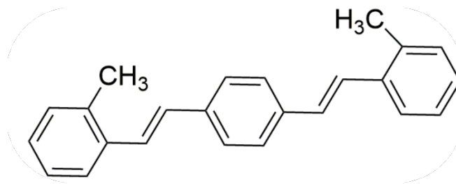
Figure 1. Structure of 1,4-bis((E)-2-methylstyryl) benzene.
