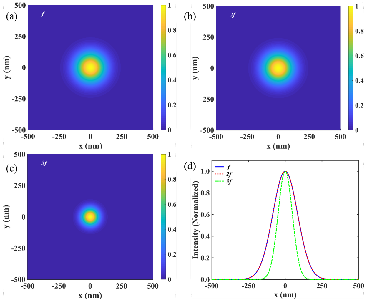
Figure 5. Calculated spatial distribution of saturated CARS signal for MSB at f (a), 2f (b), 3f (c), and the intensity profile (d). The FWHM determined from the intensity profile is 200 nm for both f and 2f . It is 116 nm for 3f . The beam width parameters ( \sigma_j ) for the pump beam ( \lambda = 885.6 nm) and Stokes beam ( \lambda = 1031 nm) were 111 nm and 129 nm, respectively. Other parameters used for MSB are same as those used in calculation of the saturated CARS spectra shown in Figure 4.
