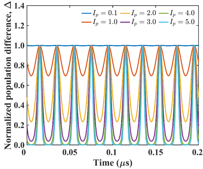
Figure 3. The effect on the population difference due to the modulation of the pump beam, at various intensities of the pump beam, for MSB. The intensity of the pump beam is given in multiples of 2.8 MW/cm 2 . The intensity of the Stokes beam was fixed at 1.6 MW/cm 2 . The
