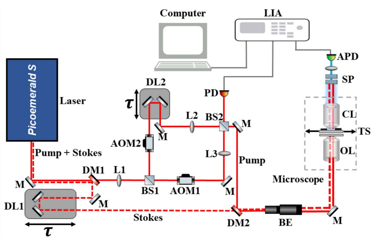
Figure 2. The CARS apparatus. M (mirror), DM (dichroic mirror), DL (delay line), L (lens), BS (50:50 nonpolarizing beam splitter), AOM (acousto-optical modulator), BE (beam expander), OL (objective lens), TS (translation stage), CL( condenser lens), SP (short pass filter), PD (photodiode), APD (avalanche photodiode), and LIA (lock-in amplifier).
