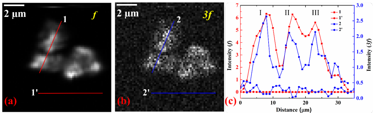
Figure 8. (a) The CARS image of diamond particles collected at f . The pump and Stokes power densities were 0.8 \text{ MW/cm}^2 and 0.5 \text{ MW/cm}^2 . (b) Saturated CARS image constructed by signal demodulation at 3f . (c) The comparison between the intensities using line profiles of two identical regions. Square markers represent intensity values for the region where diamond particles were present (1 for f and 2 for 3f ), and circular markers represent intensity values for
