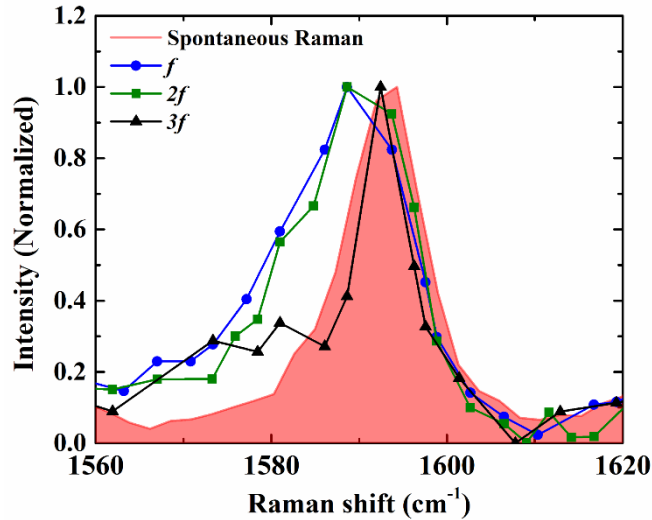
Figure 6. Comparison of experimentally obtained spectra for MSB: spontaneous Raman spectrum (pink shaded region); CARS spectra at the fundamental ( f , 500 kHz, blue) and the second harmonic ( 2f , 1MHz, olive); and the saturated CARS spectrum at the third harmonic ( 3f , 1.5 MHz, black). The pump and Stokes power densities for the CARS spectra at f and 2f were 0.8 \text{ MW/cm}^2 and 0.3 \text{ MW/cm}^2 , respectively; while for the saturated CARS spectrum at 3f , the pump and Stokes power densities were 2.8 \text{ MW/cm}^2 and 1.6 \text{ MW/cm}^2 , respectively.
