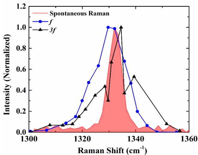
Figure 7. Spectra of diamond particles: spontaneous Raman spectrum (shaded pink region), CARS spectrum at the fundamental ( f , 500 kHz, blue), and the saturated CARS spectrum at the third harmonic ( 3f , 1.5 MHz, black). The pump and Stokes power densities for the spectrum
