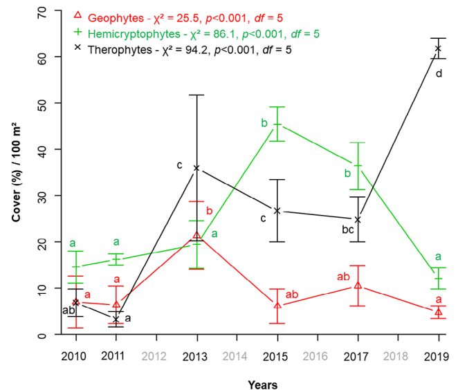
Figure 1. Mean percent cover \pm SE of plant types varying significantly between years (2010–2019) at the Carpobrotus removal site. The mean is calculated on three plots/year, located at each end of the pitfall transect and in the middle. Raunkiaer plant life forms (geophytes, hemicryptophytes, therophytes: Raunkiaer 1934) using Tison et al. (2014). The proportion of each plant type in each plot was adjusted so that the sums were equal to 100%.
