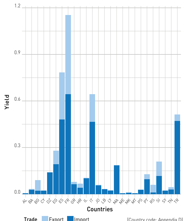
Figure 3.17 | Trade patterns in fodder and feeding products (average 2014-2017 values in tonnes x 10 6 ) in the Mediterranean countries: import (deep blue) and export (light blue) contribution for each Mediterranean country (FAO 2017).
