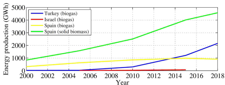
Figure 3.33 | Electricity production from biogas and solid biomass in Turkey, Israel and Spain (IEA 2018).
