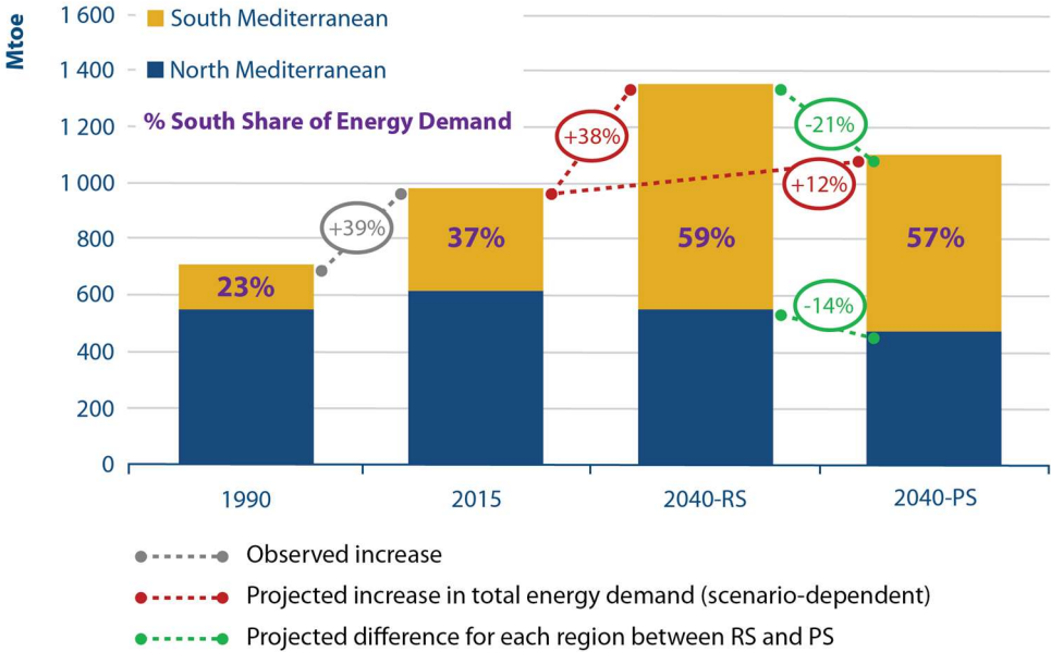
Figure 3.37 | Primary energy demand by region, in megatons of oil equivalent (Mtoe). RS = Reference Scenario; PS = Proactive Scenario (adapted from OME 2018), see Section 3.3.3.1 for definition of the scenarios.
