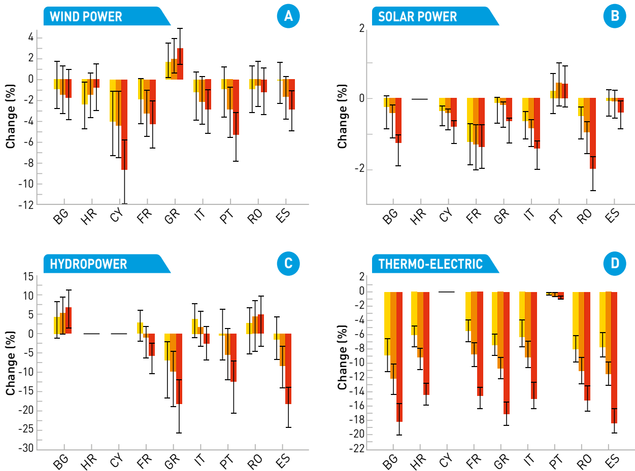
Figure 3.42 | Future changes in national wind power (A), solar PV power (B), hydropower (C) and thermo-electric power (D) production under +1.5°C global warming (yellow bars), 2°C (orange bars) and 3°C (red bars).
