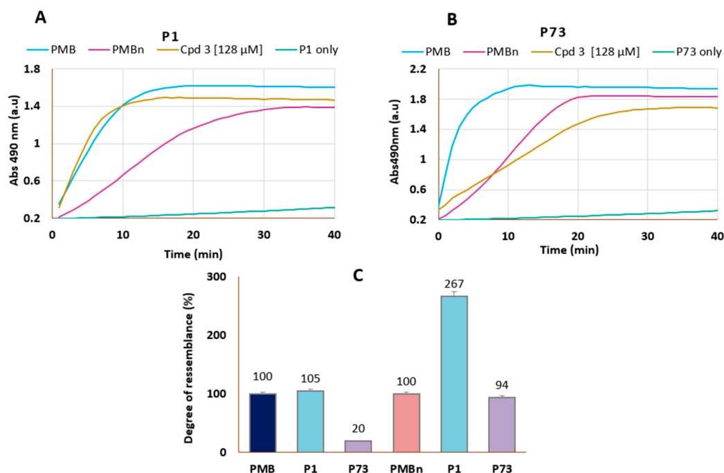
Figure 4. Study of outer membrane permeabilization of P1 (A) and P73 (B) by evaluating the rate of nitrocefin hydrolysis in the presence of PMB (200 µM), PMBn (106.3 µM), and compound 3 at 128 µM. Membrane permeation effects of compound 3 at 128 µM compared to PMB and PMBn (C).
