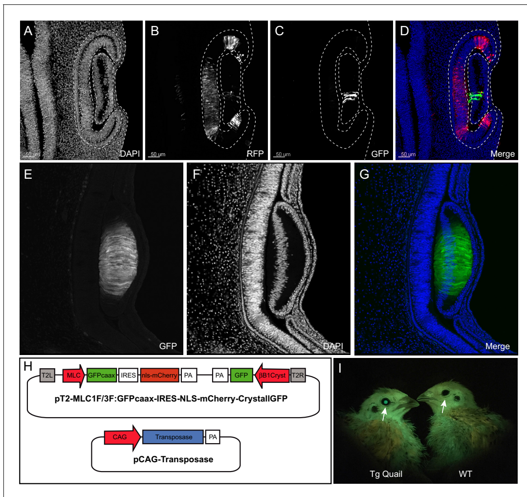
Figure 2. Design and use of the CrystallGFP mini gene. (A–D) Cross-section of the head of an E4 embryo, electroperated one day earlier in the optic cup with a CrystallGFP minigene. (A) DAPI, (B) electroporation marker CAG-RFP plasmid, (C) GFP, (D) overlay. (E–G) Cross-section of the head of a 3-day-old embryo of the Tg(MLC:GFP-IRES-NLS-mCherry,CRYBB1:GFP) transgenic line showing the specific expression of GFP throughout the lens. (H) Electroperation constructs used to express the CrystallGFP minigene in a muscle-specific transgenic line (see Figure 4 ). (I) Transgenic and WT adults of the muscle-specific transgenic line showing GFP expression in lens.
